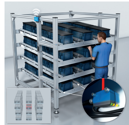
Automated material reordering at e-Kanban racks
