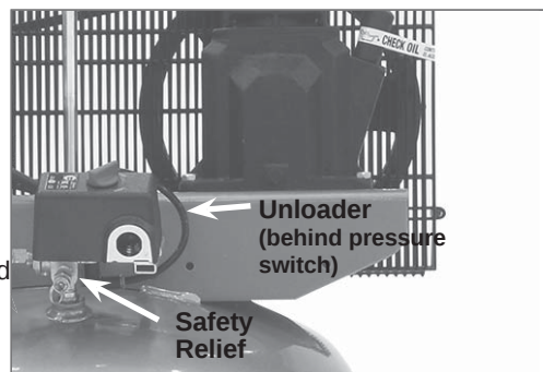
Figure 7 - Pressure Switch
