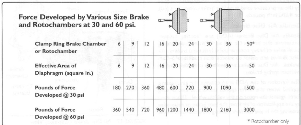
FIGURE 15 - Braking Forces-Effect of Brake Chamber Size
