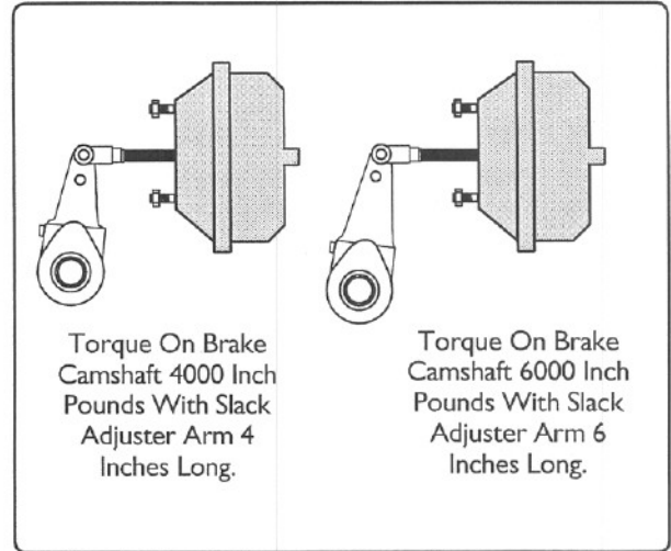
FIGURE 16 - Braking Forces-Effect of Slack Adjuster Arm Length
