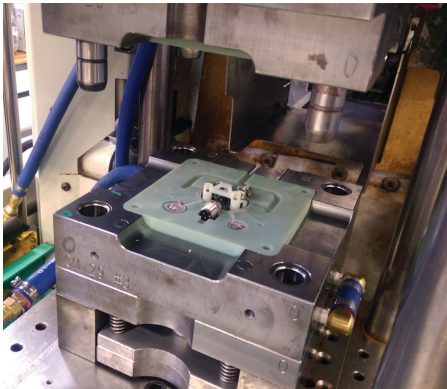
3D printed mold in the press
