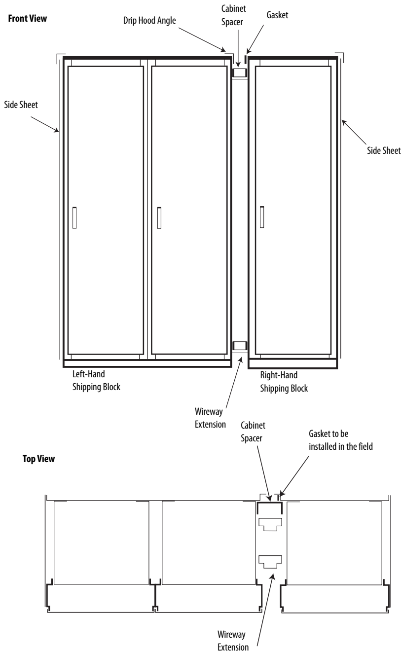
Figure 5 - NEMA 3R/4
