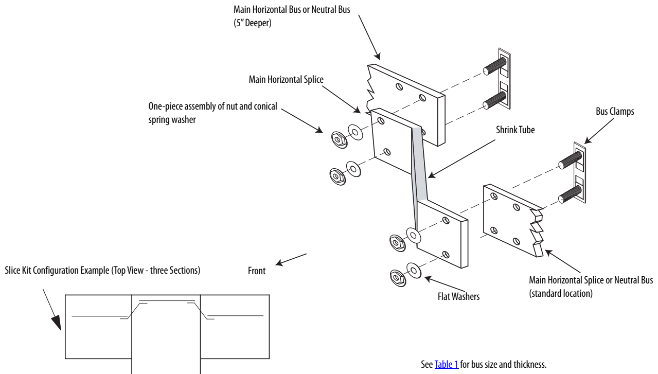
Figure 15 - 25 in. Deep 'Z' 600...1200 Amp Bus Splicing Detail and Configuration Example
