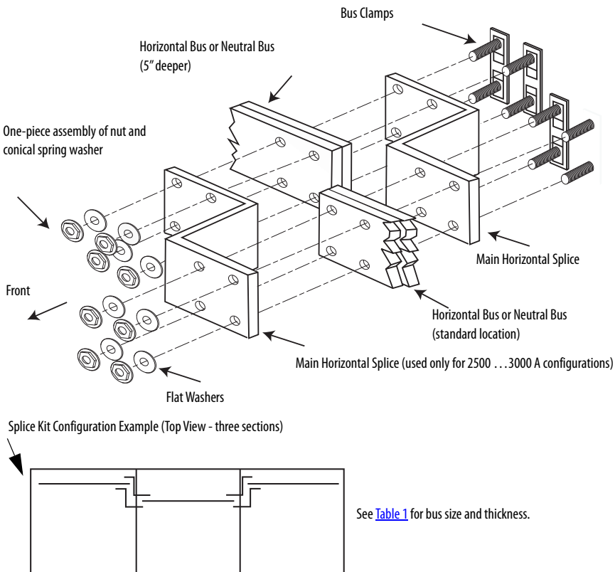
Figure 14 - Offset 'Z' 1600...3000 Amp Bus Splicing Detail and Configuration Example
