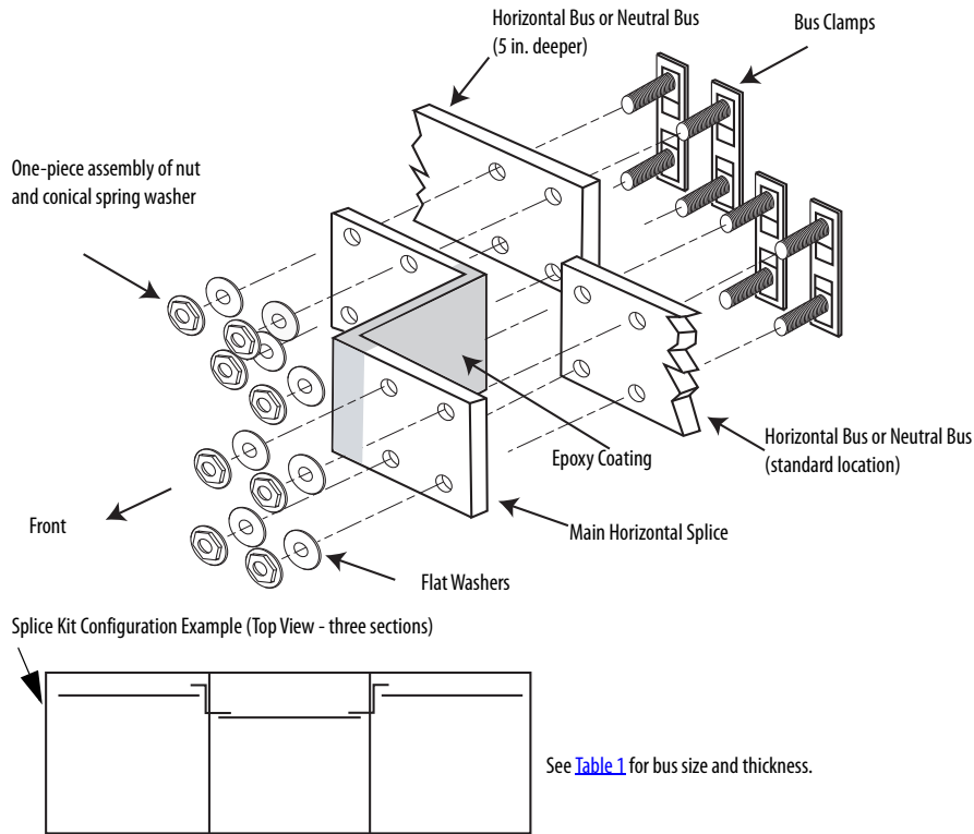
Figure 14 - Offset 'Z' 1600...3000 Amp Bus Splicing Detail and Configuration Example
