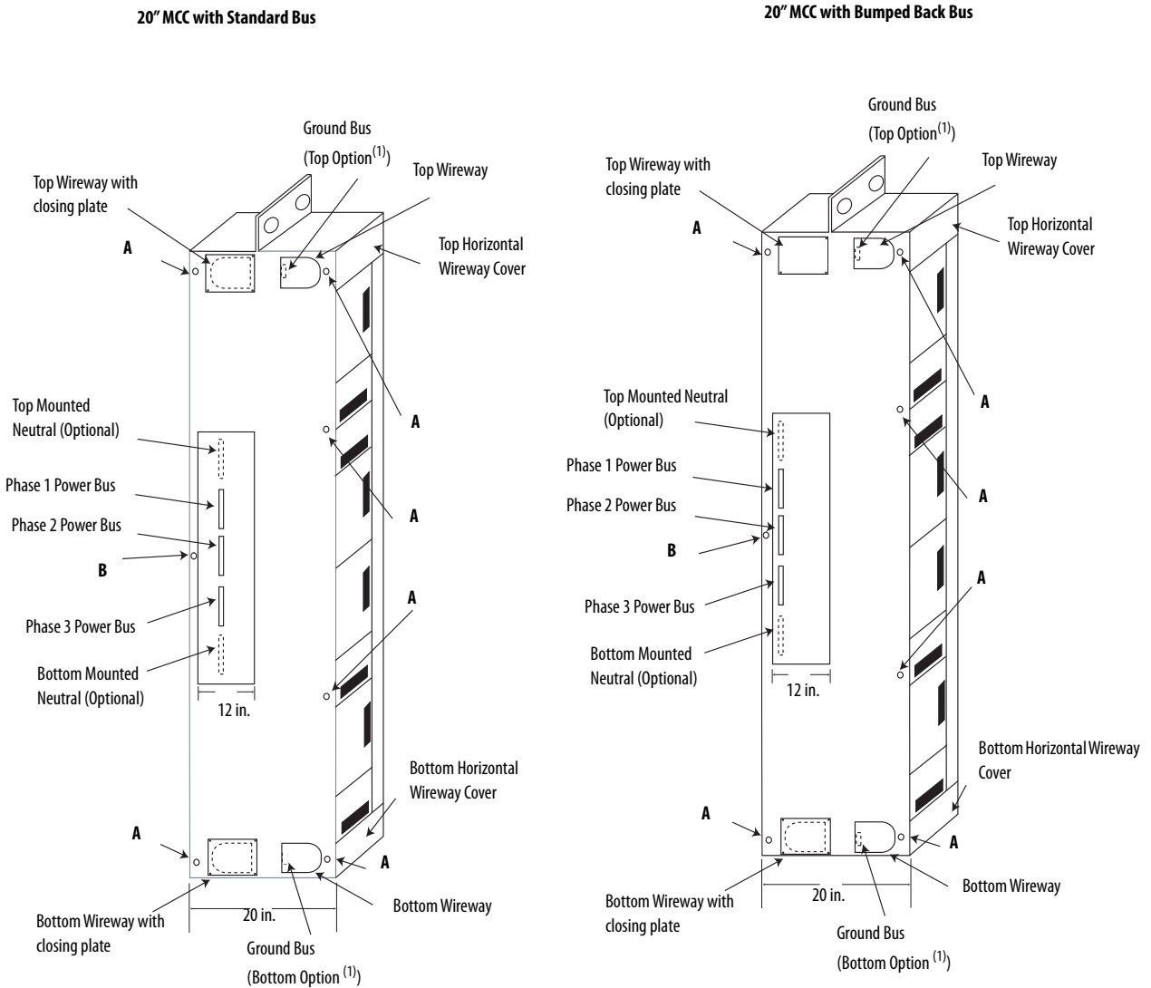
Figure 3 - Example of 20" Deep MCCs
