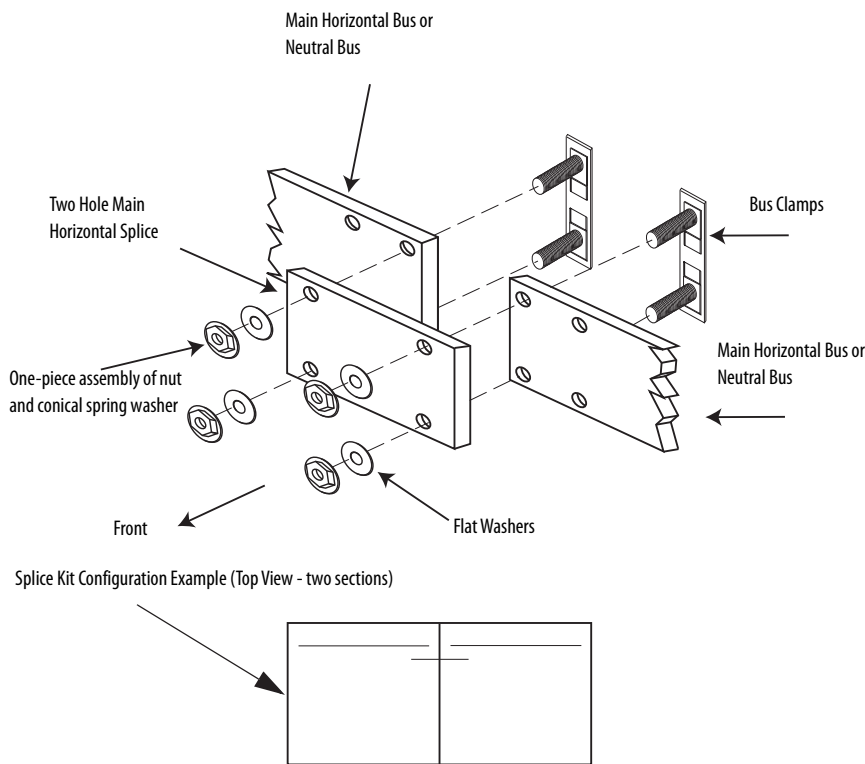
Figure 8 - 600...1200 Amp Main Horizontal Bus Splicing Detail and Configuration Example
