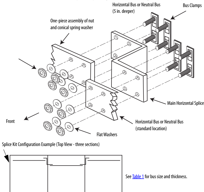
Figure 12 - Offset 'Z' 600...1200 Amp Bus Splicing Detail and Configuration Example
