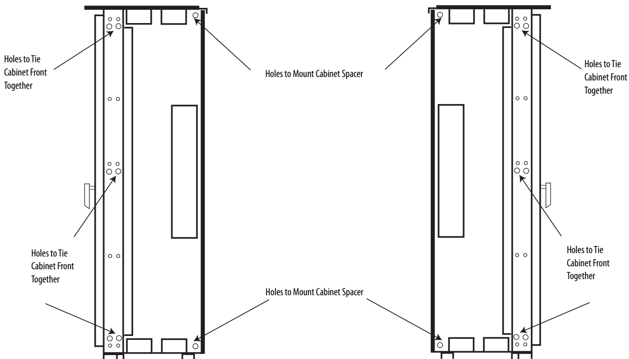
Figure 4 - NEMA 3R/4 without Side Sheet.
