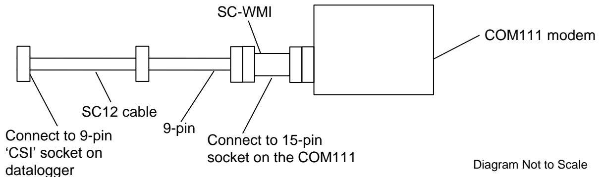
Figure 1. Connecting the COM111 modem to a Datalogger using an SC-WMI
