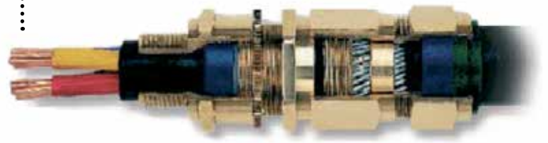
Cutaway of typical cable gland
