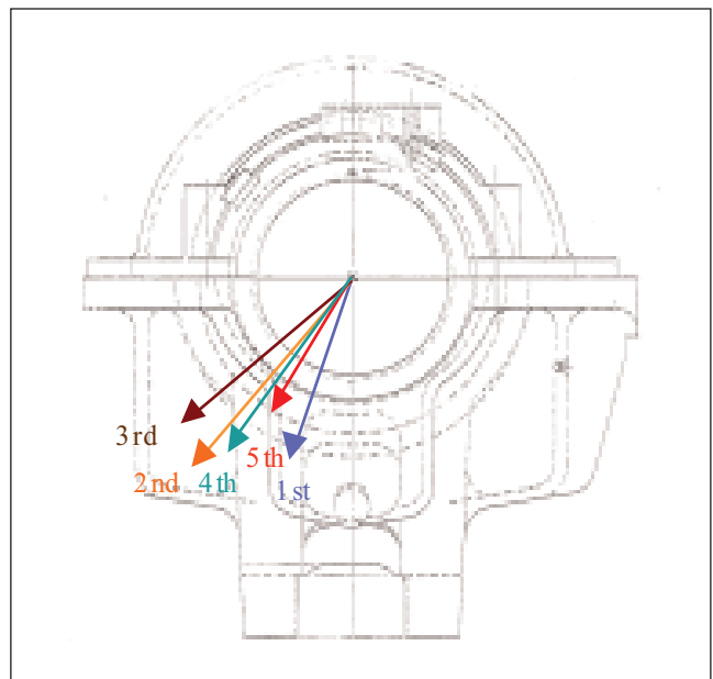
Figure 10. Sketch of bearing with partial arc valve forces for each valve point. Vector magnitudes are to scale relative to each other.
