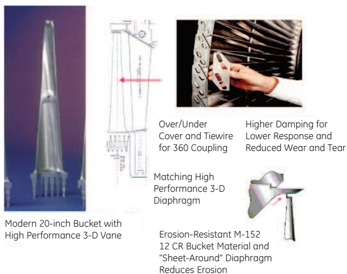
Figure 4. 3D 20-inch last stage bucket and diaphragm
