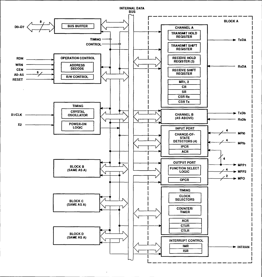
SCC2698B – BLOCK DIAGRAM
