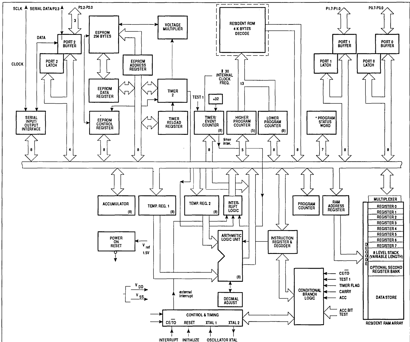
PCD3346 - BLOCK DIAGRAM
