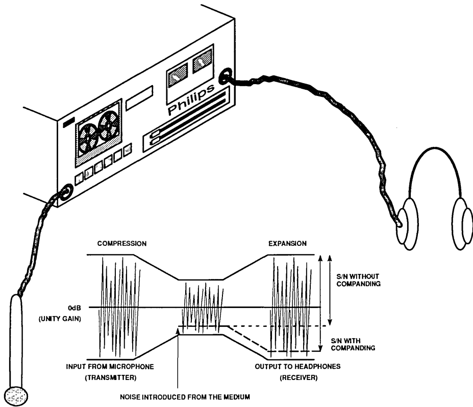
Application diagram shows a compandor's function
