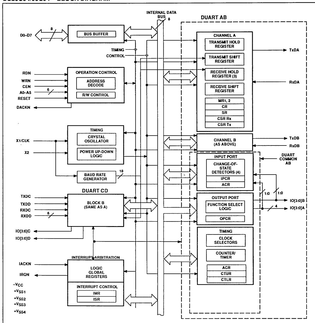
SC26C94/68C94 – BLOCK DIAGRAM
