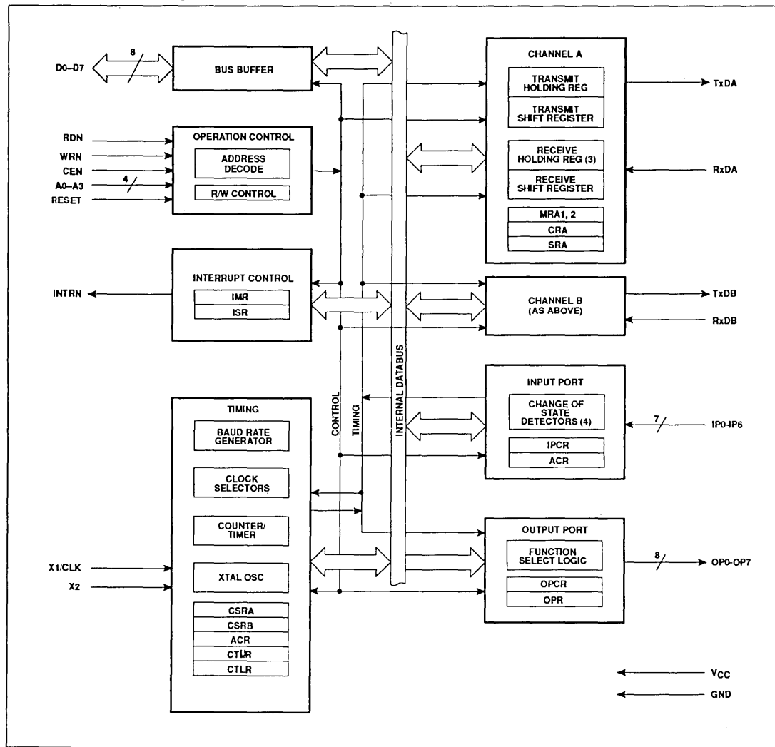
SCC2692 – BLOCK DIAGRAM
