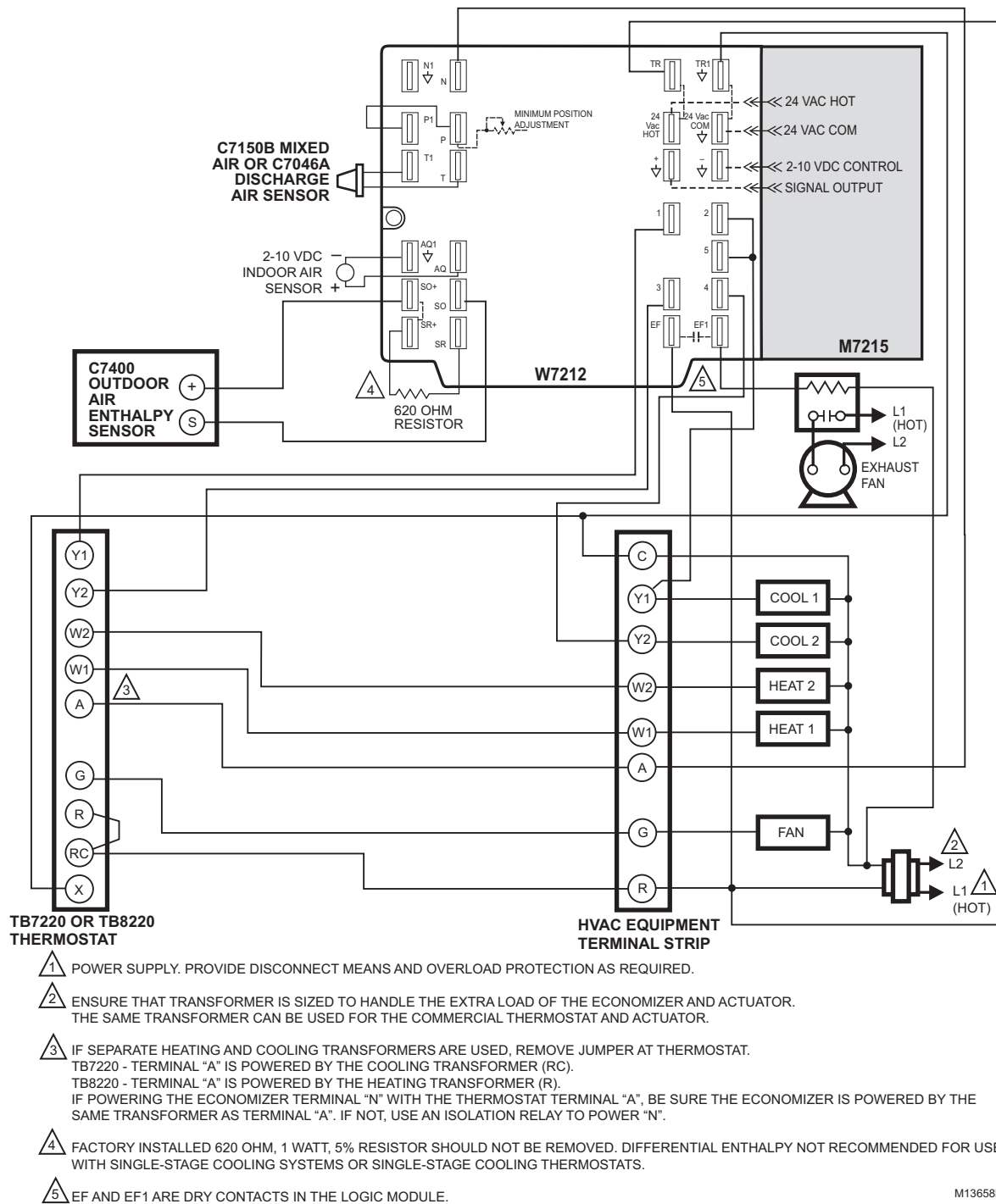
Fig. 11. W7212 used with M7215 Damper Motor and TB7220 or TB8220 Thermostats.
