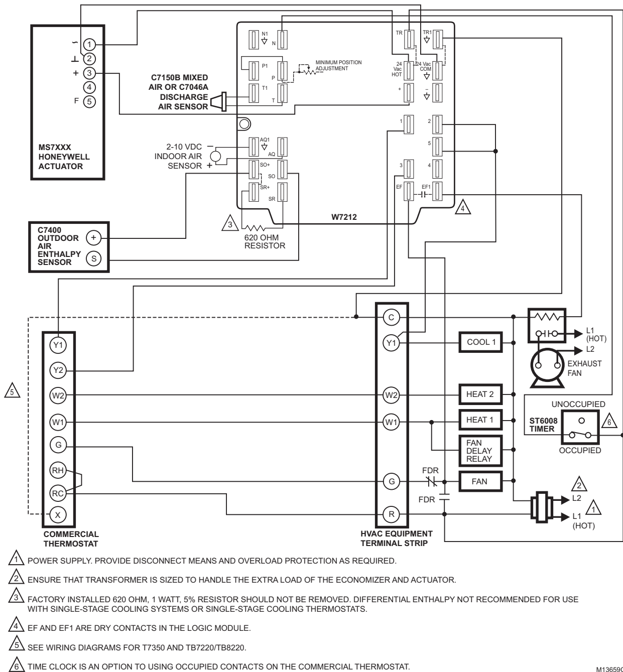
Fig. 12. W7212 used in single-stage cooling system with single enthalpy changeover and Honeywell actuator and time clock for occupancy.
