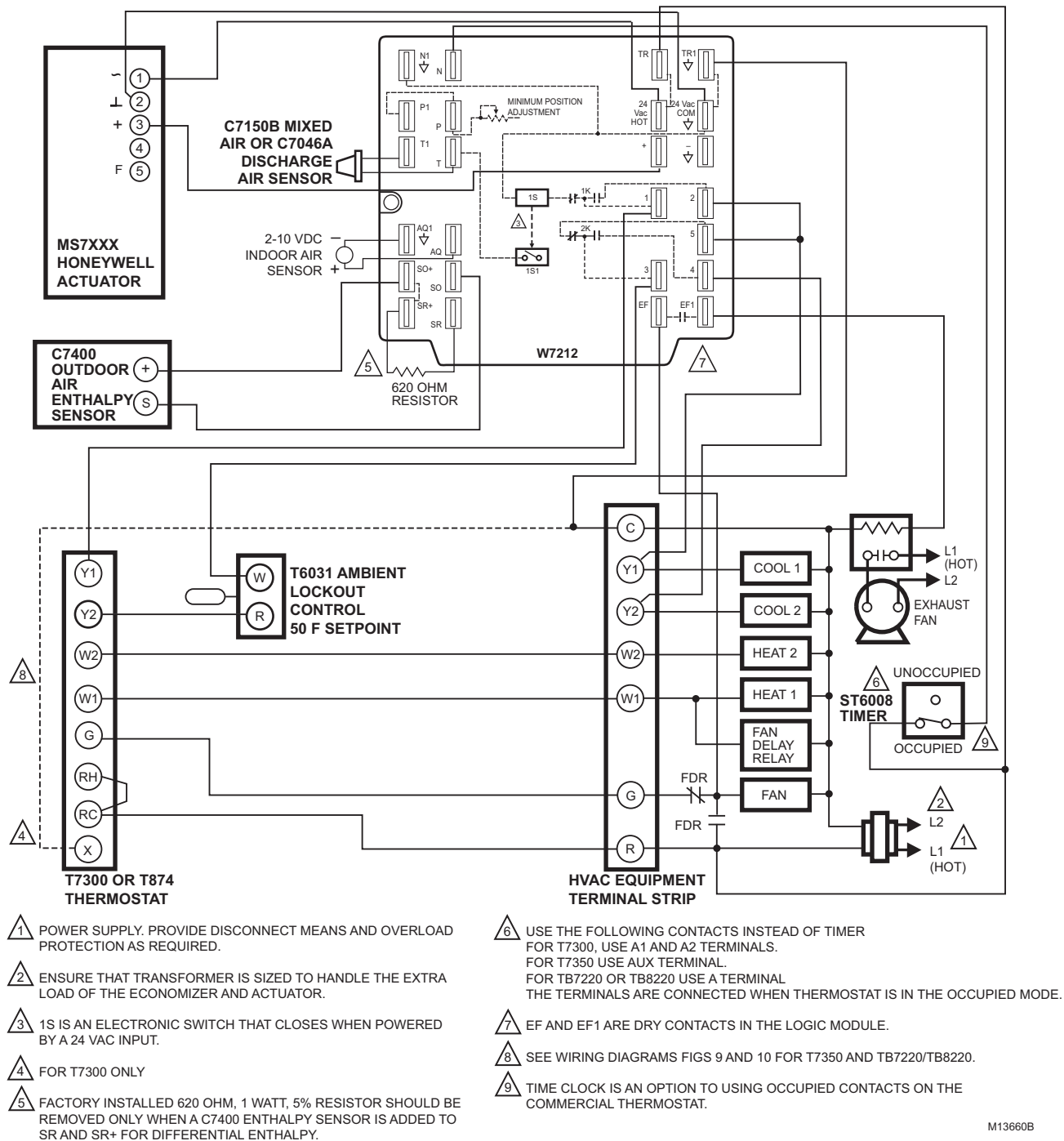
Fig. 13. W7212 used in two-stage cooling system with Honeywell Series 72 Actuator and time clock for occupancy.
