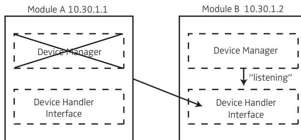
Figure 18. Example 2
