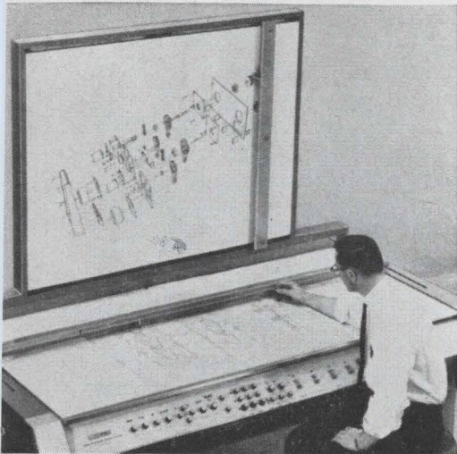
Drawing machine uses computer to convert orthographic drawings into three-dimensional sketches at any perspective.
