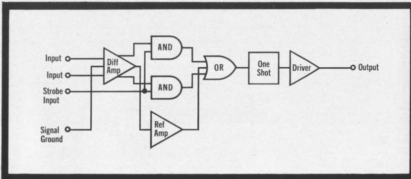
Figure 1. Functional diagram shows that the SN5500 is a complete sense amplifier, including differential preamplifier, reference amplifier, strobe gate, and pulse-shaping output circuit.
