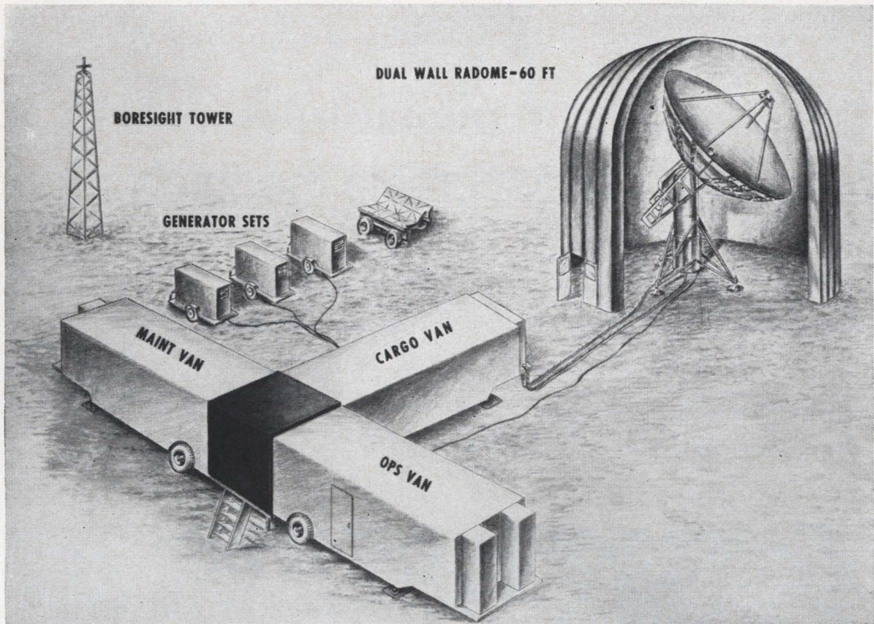
The air-transportable communications terminal, AN/MS-46, consists of three vans, three generator sets, a boresight tower, and a 40-foot antenna enclosed in a dual wall radome.
