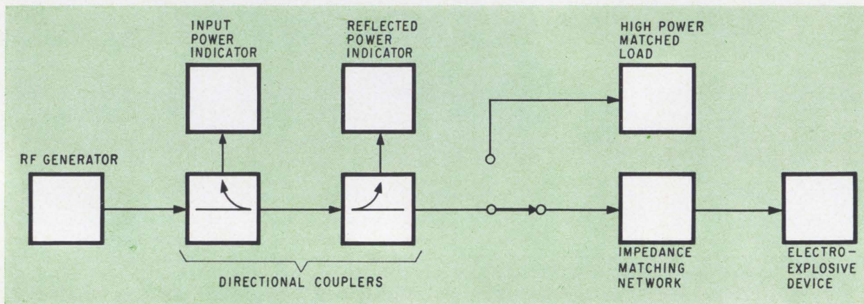
Attenuation of ferrite and powdered iron samples were measured by the "sample substitution" technique shown in the diagram at the top. Sample attenuation is the difference in the galvanometer power reading when an air line or sample is inserted in the system. The system in the lower diagram measures the r-f power necessary to fire the electroexplosive devices by comparing r-f power levels in ideal and real loads.
