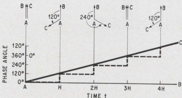
Crystal oscillator output (line AC) advances continuously 120^\circ in phase during each horizontal line (time H ) with respect to the transmitted reference subcarrier burst, (line AB). The oscillator's output phase, however, must be kept constant during each time H (as shown by the dotted line and the phasors) to provide axes for demodulation. This is done by phase modulating the oscillator output in the opposite direction to its phase advance for a period H .
