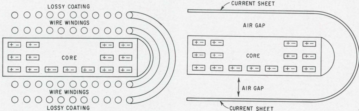
Cross-section of inductor (left) with wire windings and magnetic dipoles oriented in the core. Simplified drawing at right shows how current passing through the wire can be visualized as a sheet of current flowing around the core. The key to making miniature inductors lies in reducing the air-gap space by bringing the sheet current closer to the core, thus obtaining better orientation of the magnetic dipoles.
