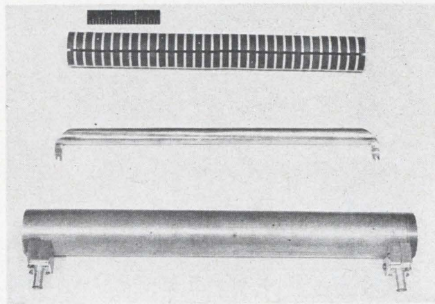
Disassembled view of variable delay line shows dielectric stack of slotted ferrite and ceramic disks (top), inner conductor (center) and outer conductor (bottom). Time delay variation is continuous, but characteristic impedance is constant.
