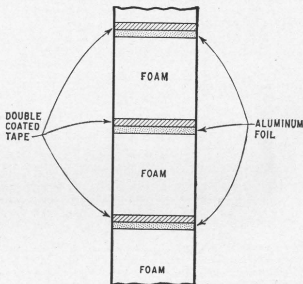
Styrofoam in a lens "sandwich" can be easily cut to tolerances of 0.01 inches for accurate spacing between foil strips. Strip width and spacing is a function of the radar frequency.
