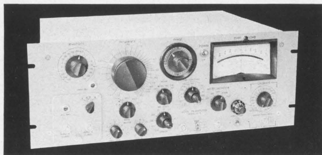
Transistorized Lock-In Amplifier — Model HR-8
