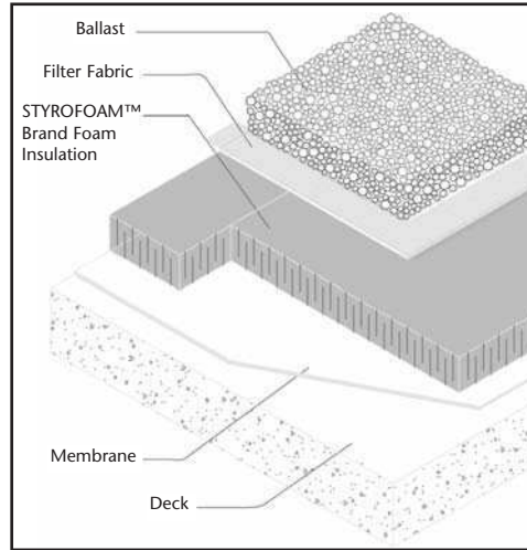
Figure 3: Fabric Placement**
