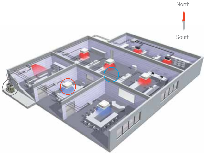
Refrigerant piping
