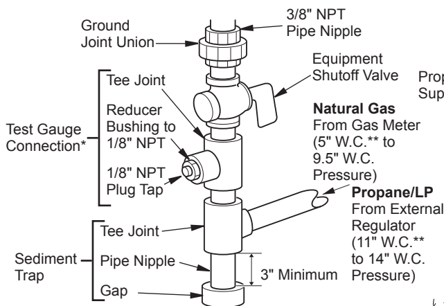
Figure 15 - Gas Connection
