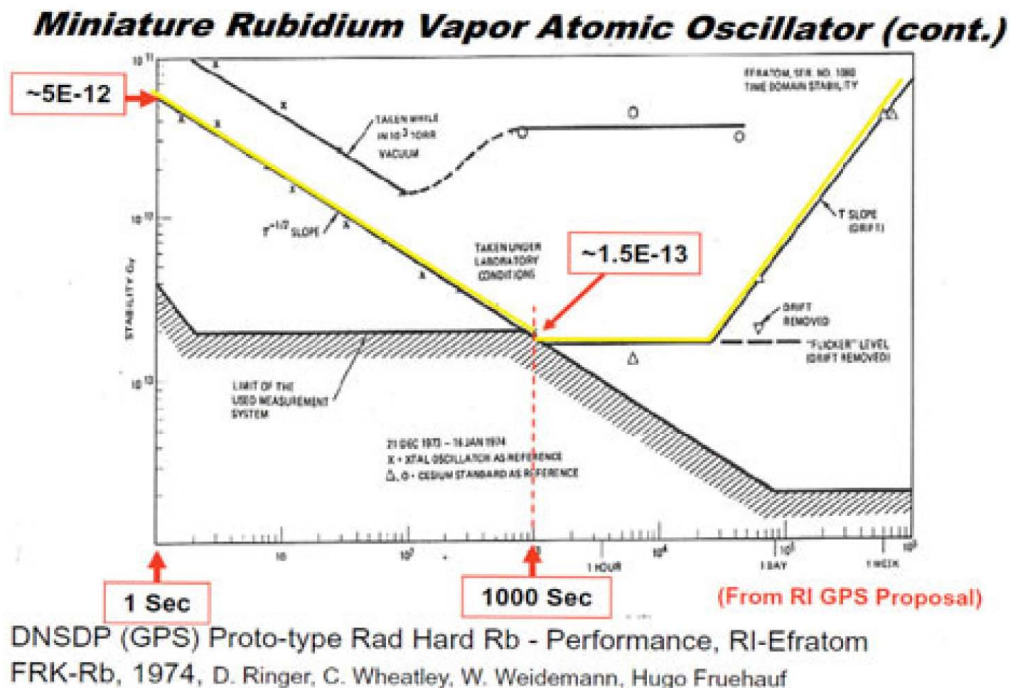
Figure 2. Test results for the Rockwell proposed GPS space-hardened prototype atomic (rubidium) clock, based on the Efratom commercial clocks.
