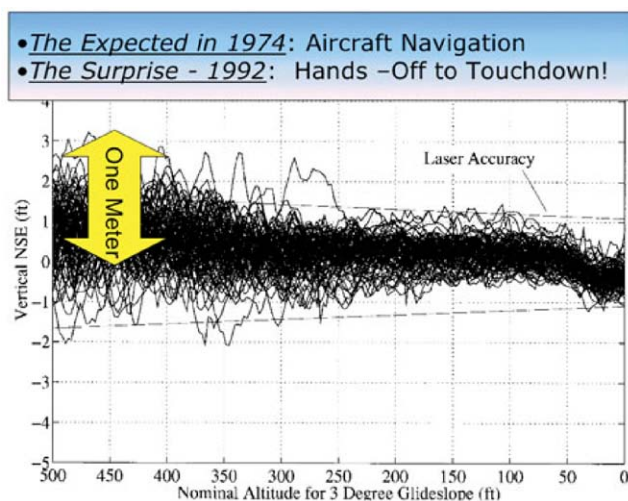
Figure 6. Results of first blind landing tests using GPS alone, 110 landings with a commercial Boeing 737.
