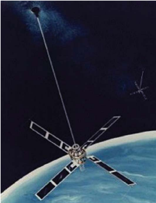
Figure 3. A Transit satellite showing the gravity-gradient boom that kept the antennas pointing at the earth.
