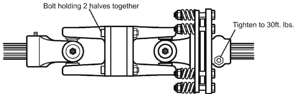
Clutch End to Center Section Gearbox
