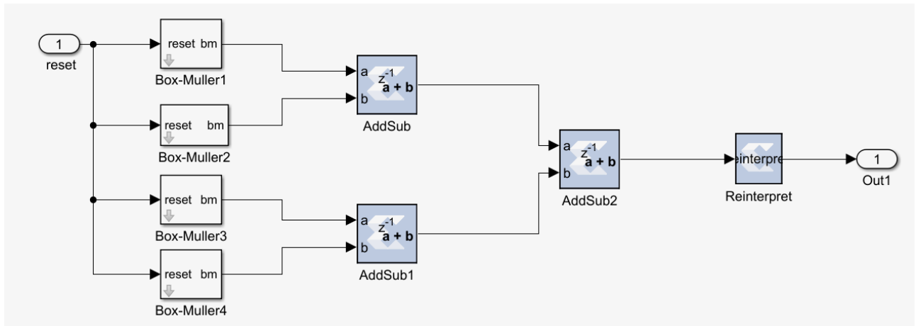
Figure 107: Box-Muller Method Diagram
