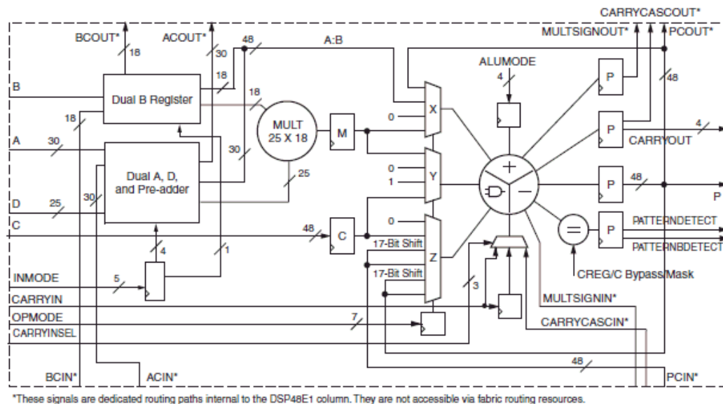
Figure 26: DSP48E1
