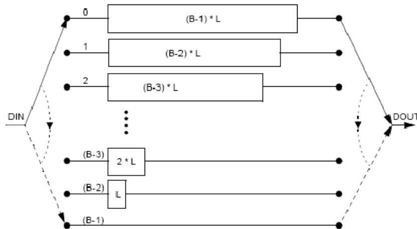
Figure 34: De-interleaver
