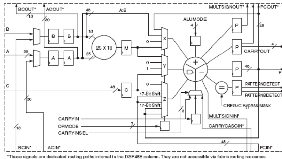
Figure 25: DSP48E
