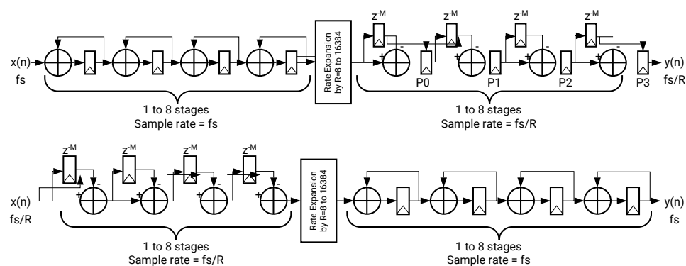
Figure 91: CIC Filter
