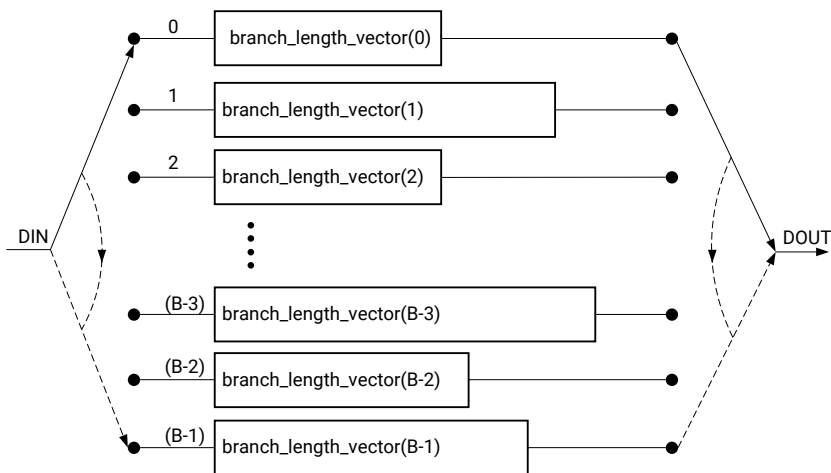
Figure 35: Interleaver/De-Interleaver
