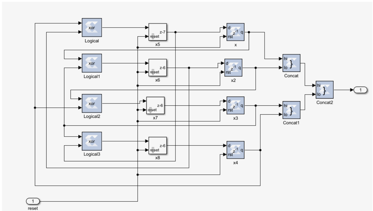
Figure 106: 4-bit Leap-Forward LFSR Diagram
