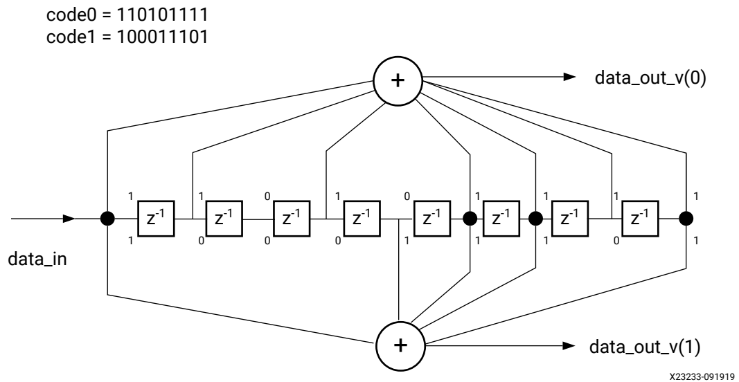
Figure 92: Encoder Rate
