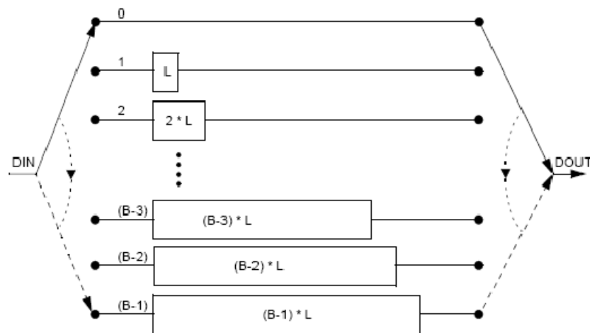
Figure 33: Interleaver
