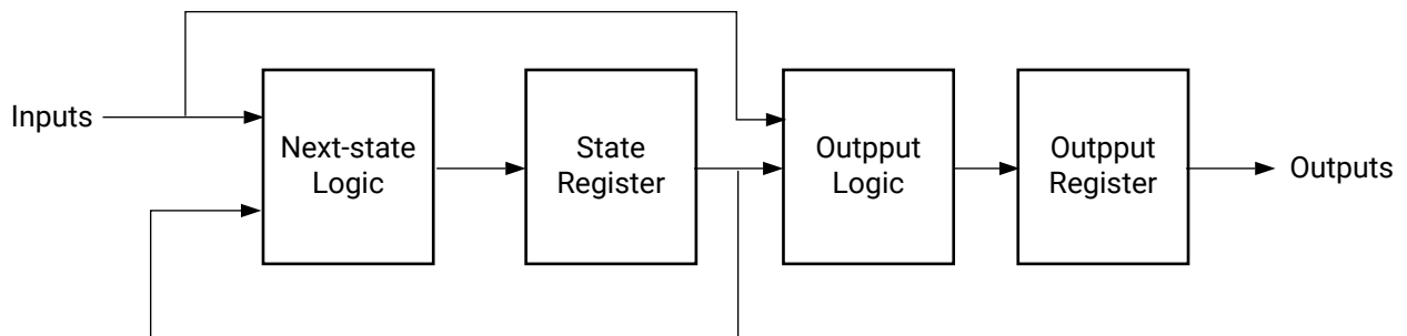
Figure 100: Mealy State Machine Block Diagram
