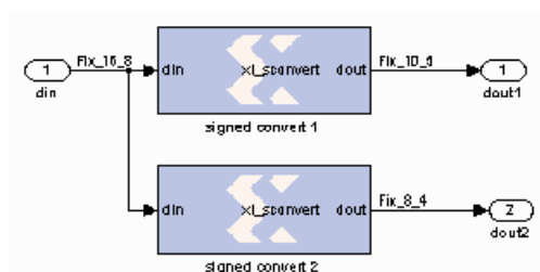
Figure 51: Block Diagram
