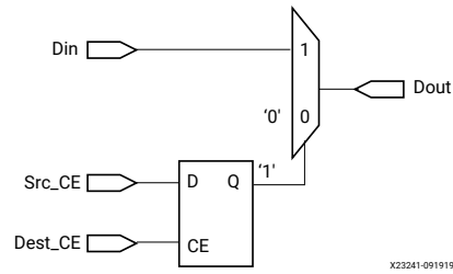
Figure 88: Zero Padding Up Sample Circuit
