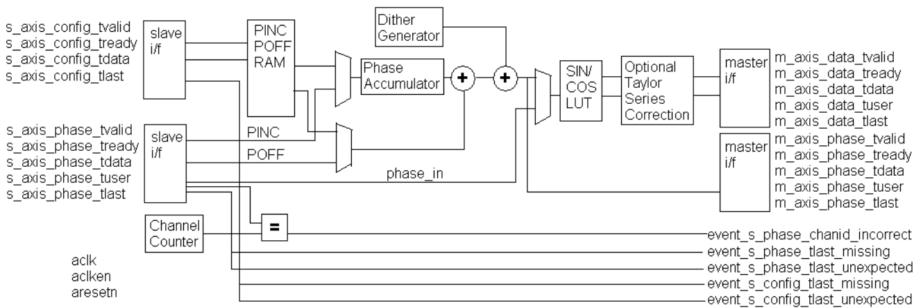
Figure 12: DDS Compiler Block Diagram
