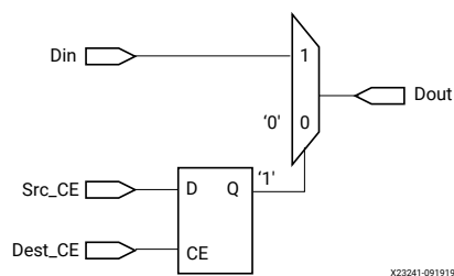
Figure 78: Zero Padding Up Sample Circuit
