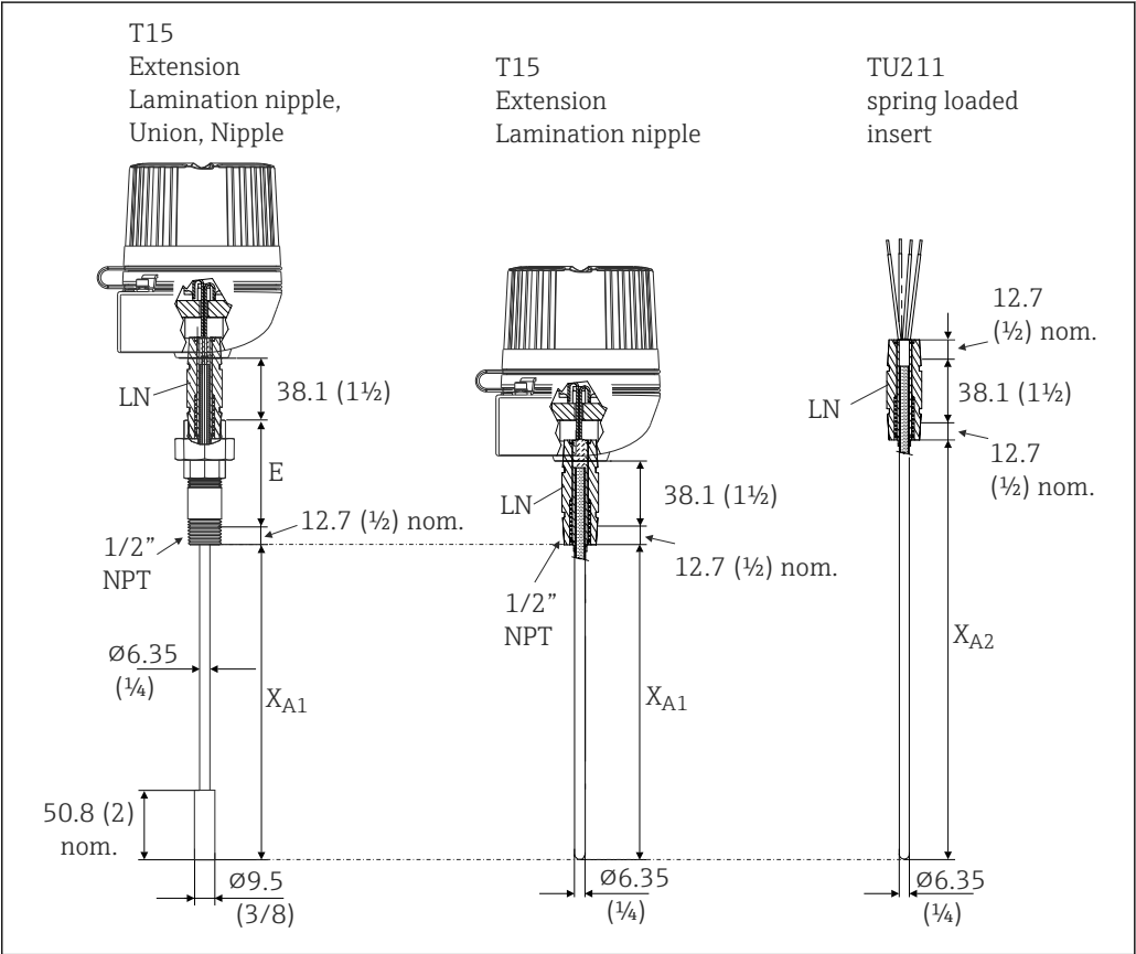
4 Design and dimensions of T15 (without thermowell), all dimensions in mm (in)
