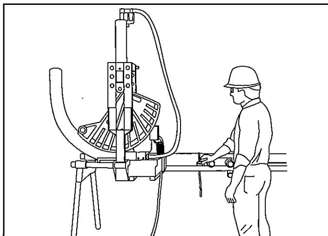
52. Release the vise chain.
