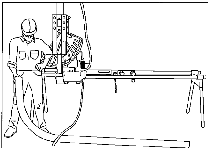
54 and 55. The 90° bend is complete.
