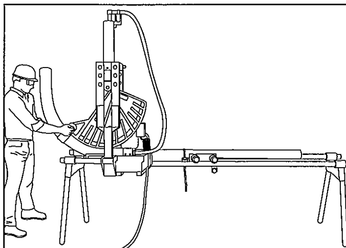
51. Remove the saddle pin and saddle.
