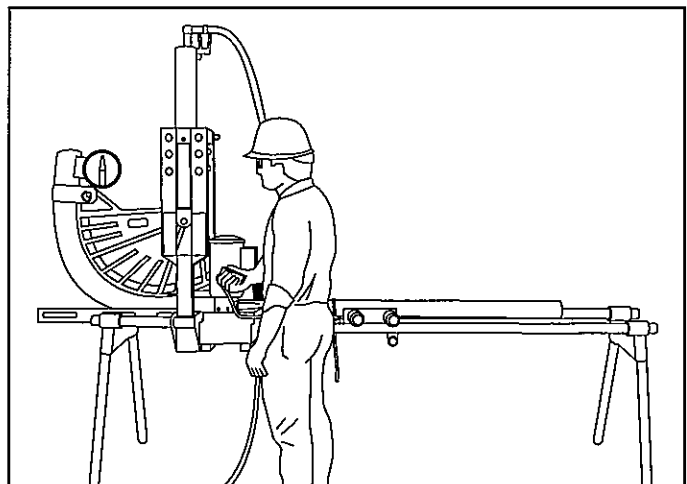
46. 75° of bend.
