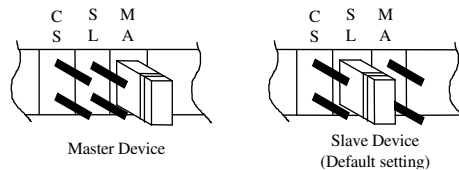
Figure: Setting the Master/Slave jumper.
