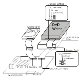
Figure: Configuration (B-2)
