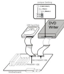
Figure: Configuration (A)
