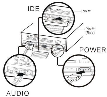
Figure: Connecting Cables
