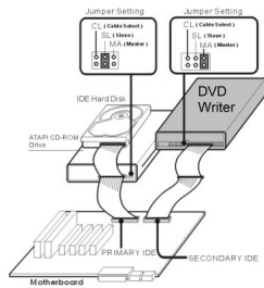
Figure: Configuration (B-1)
