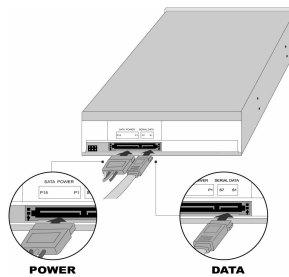
Figure: Rear Panel of Serial ATA Drive
