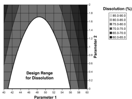
Figure 2b: Contour plot of dissolution as a function of Parameters 1 and 2.
