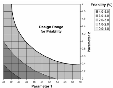
Figure 2a: Contour plot of friability as a function of Parameters 1 and 2.
