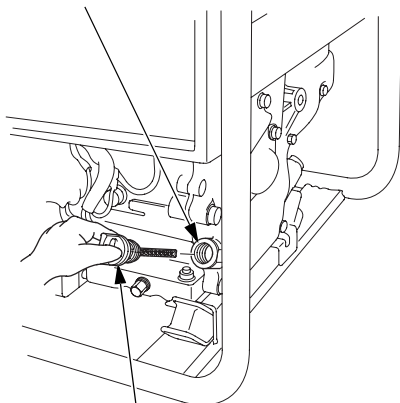
OIL FILLER NECK
