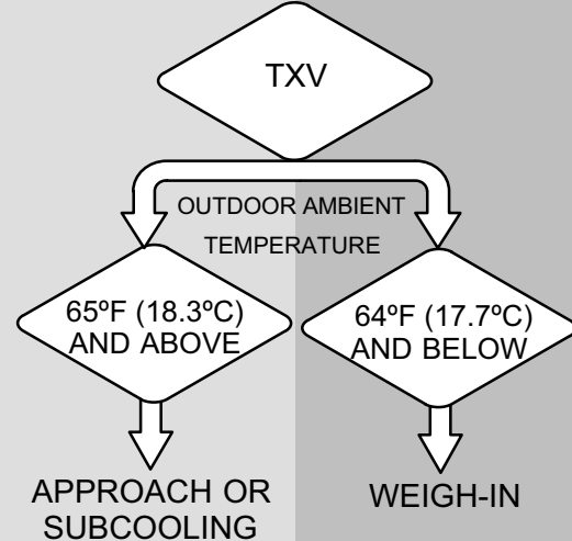
Figure 17. Determining Charge Method
