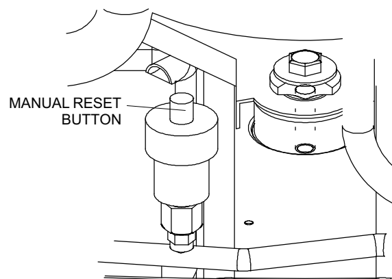
Figure 22. High Pressure Switch (S4) Manual Reset LOW PRESSURE SWITCH (S87)
