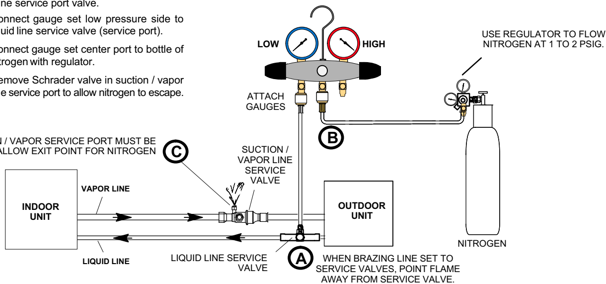
Figure 8. Brazing Procedures
