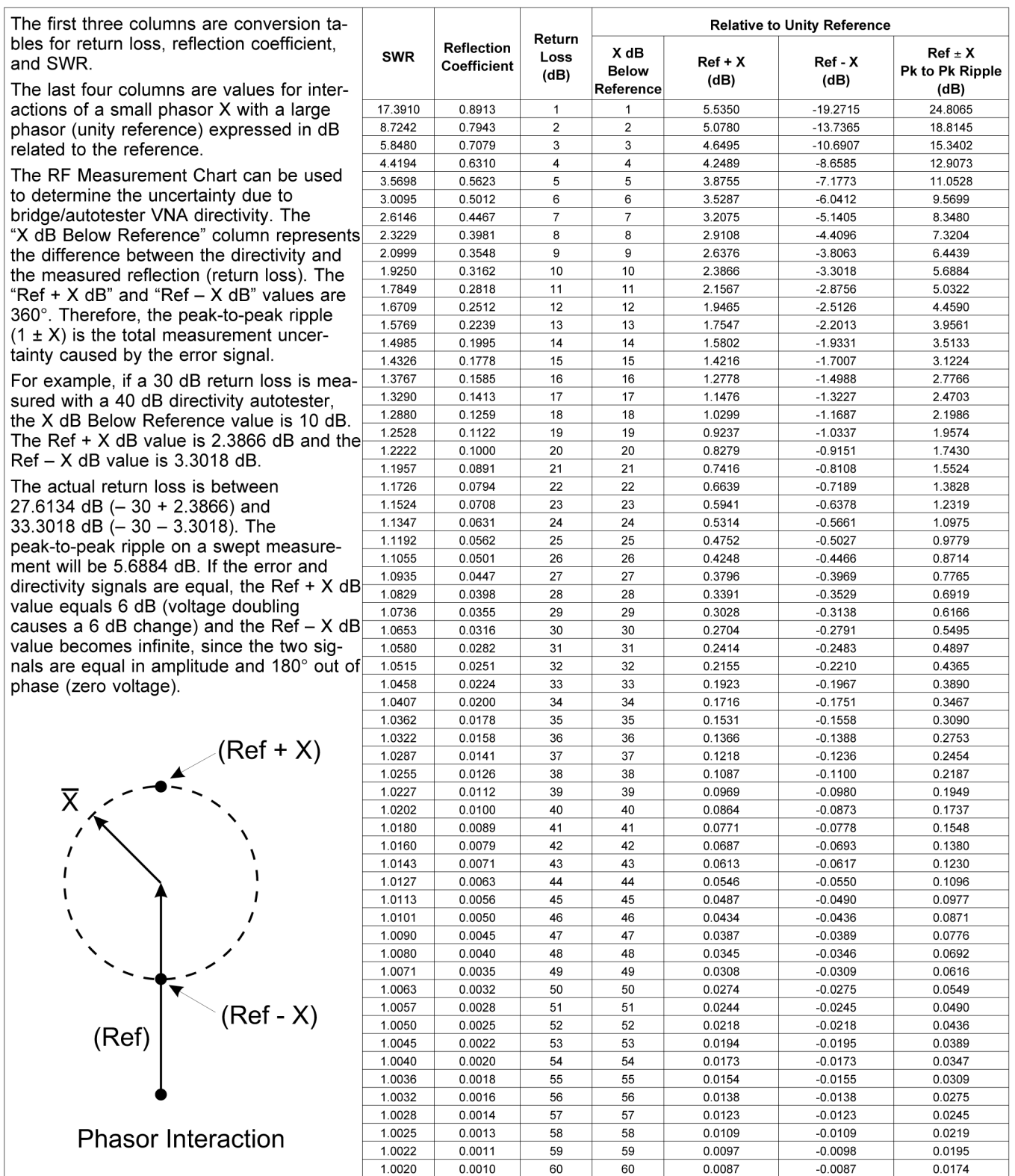
Figure 3-3. RF Measurement Chart
