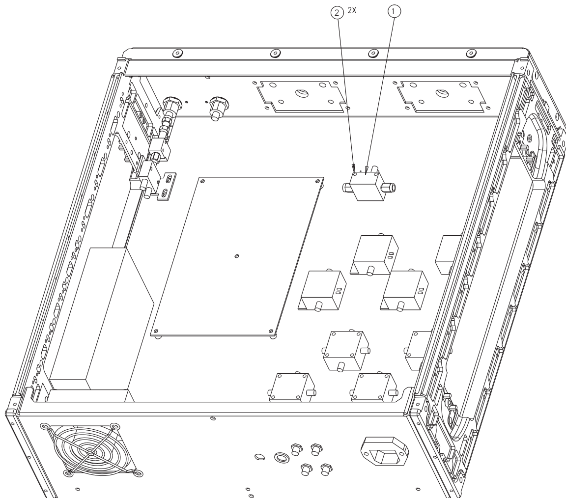
Figure 6-6. Transfer Switch Removal
