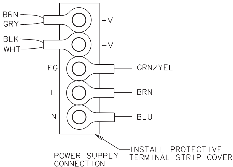
Figure 6-3. Power Supply Cable Connection
