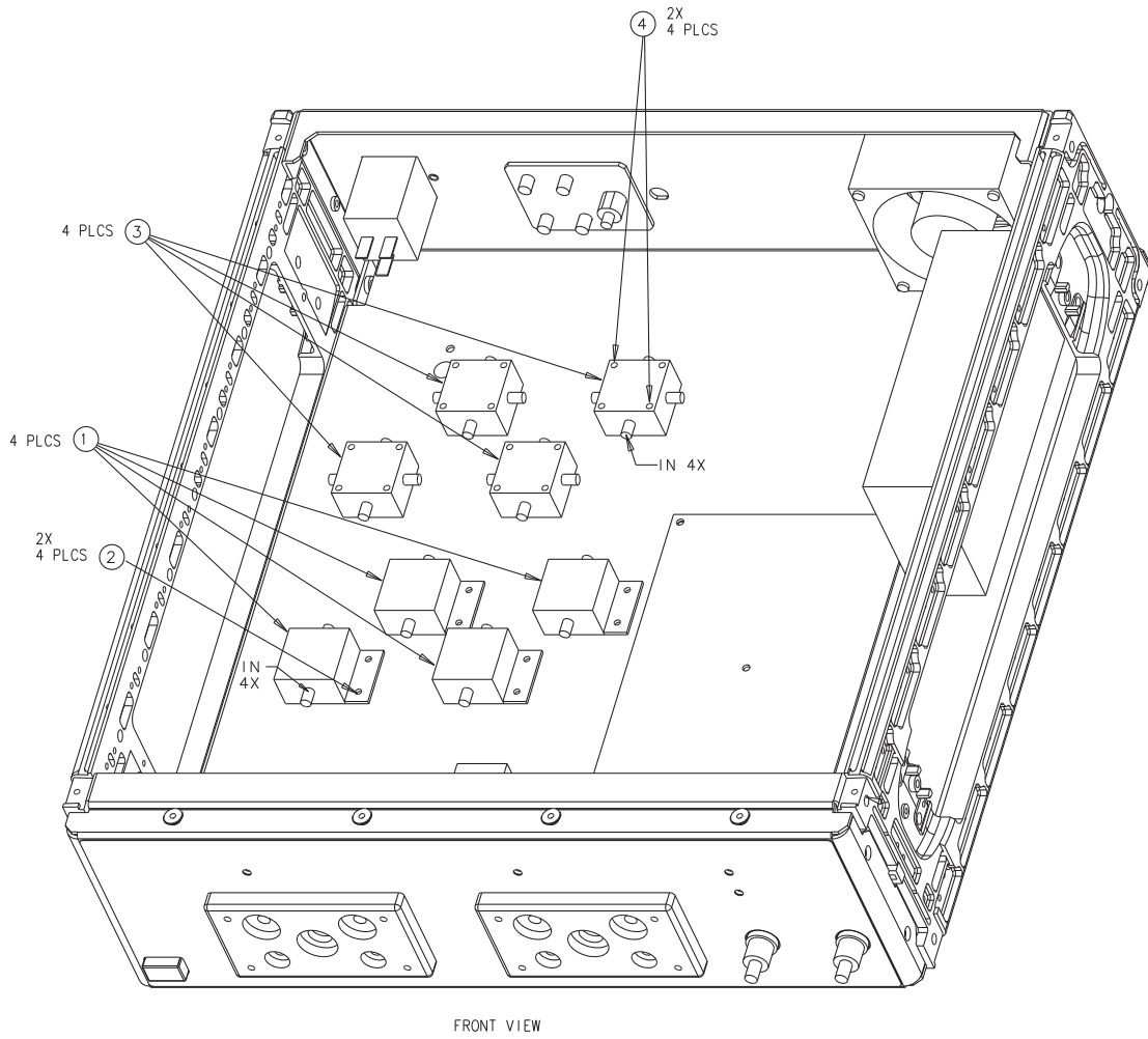
Figure 6-7. IF Amplifier and IF Switch Removal
