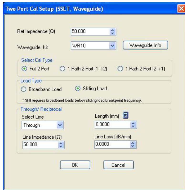
Figure 3-1. Two Port Cal Setup window
