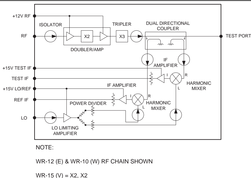
Figure 4-2. Block Diagram of 3740A-X Transmission/Reflection Millimeter-Wave Module
