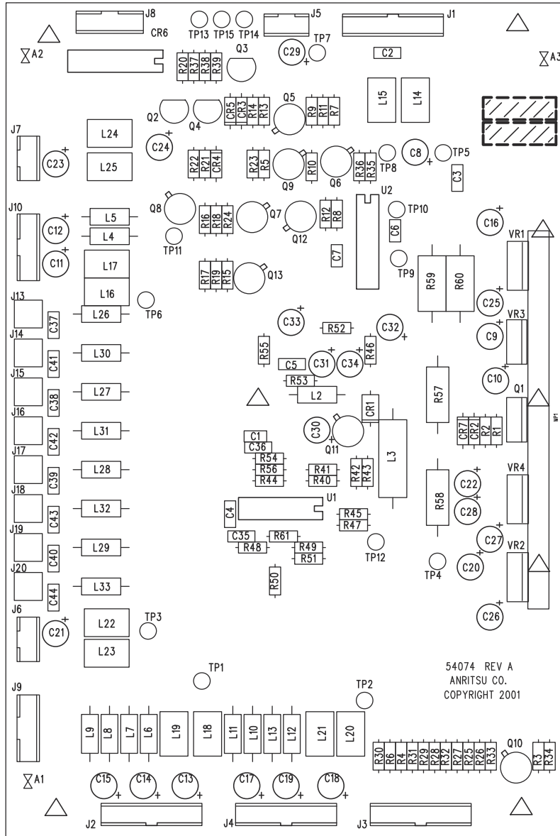
Figure 5-1. Control PCB Assembly Test Point Locations
