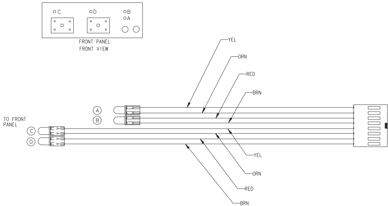
Figure 6-9. Front Panel LED Cable Assembly
