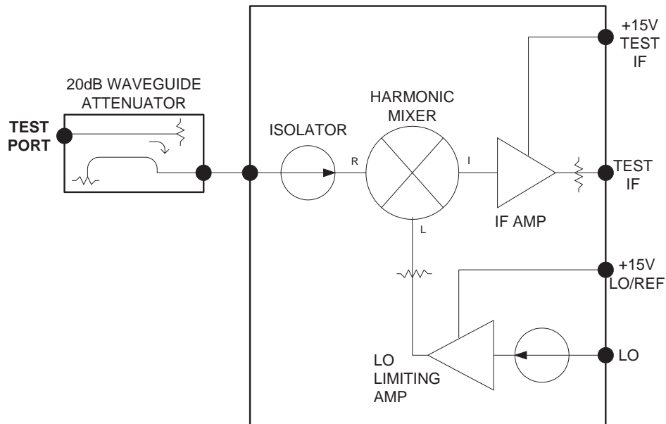
Figure 4-3. Block Diagram of 3741A-X Transmission Module
