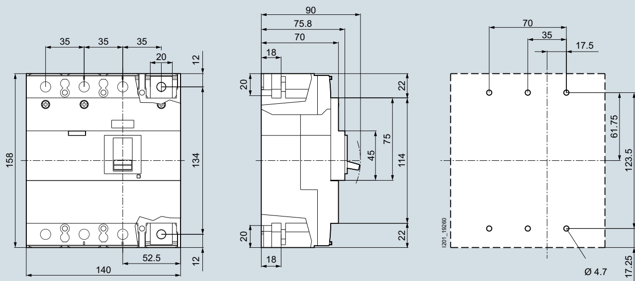
3VM12, 4 polos
