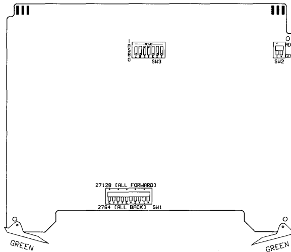
Figure 6-1. EPROM Memory Card Switches
