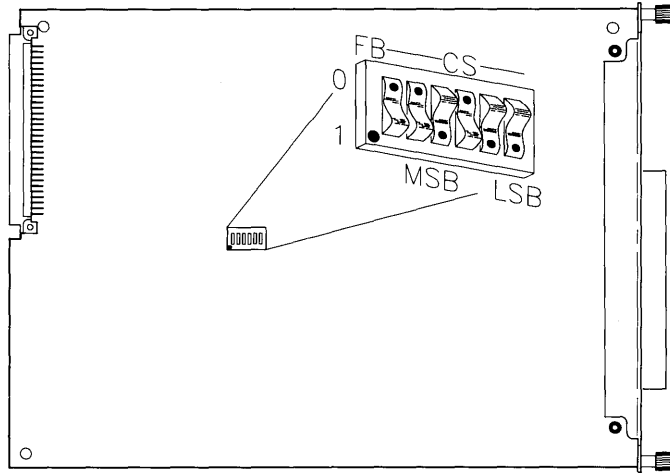
Figure 5-25. HP 98725A LGB Interface Switches
