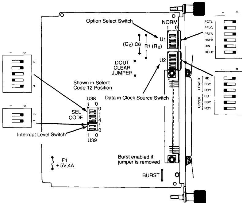
Figure 5-5. HP 98622A GPIO Switches and Jumpers
