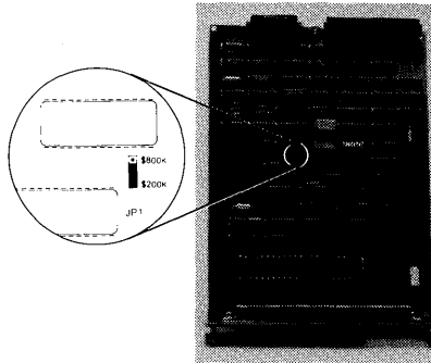
Figure 5-27: HP 98726A Jumper #1 Default Position
