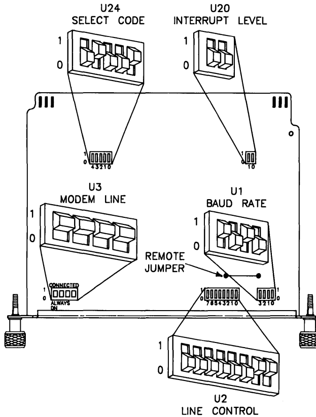
Figure 5-10. HP 98626A RS-232C Serial Interface Switches
