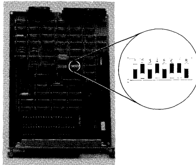
Figure 5-26: HP 98726A Interface Switches
