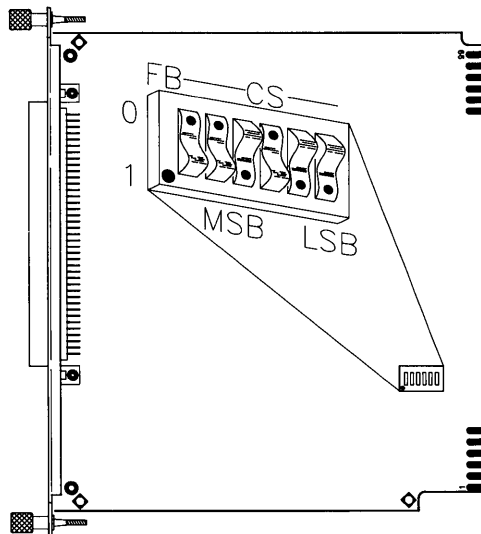
Figure 5-24. HP 98724A LGB Interface Switches
