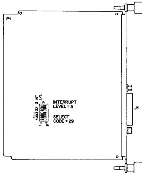
Figure 5-13. Multiprogrammer Interface Switches
