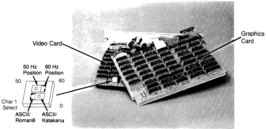
Figure 5-3. Display Compatibility Interface switches.
