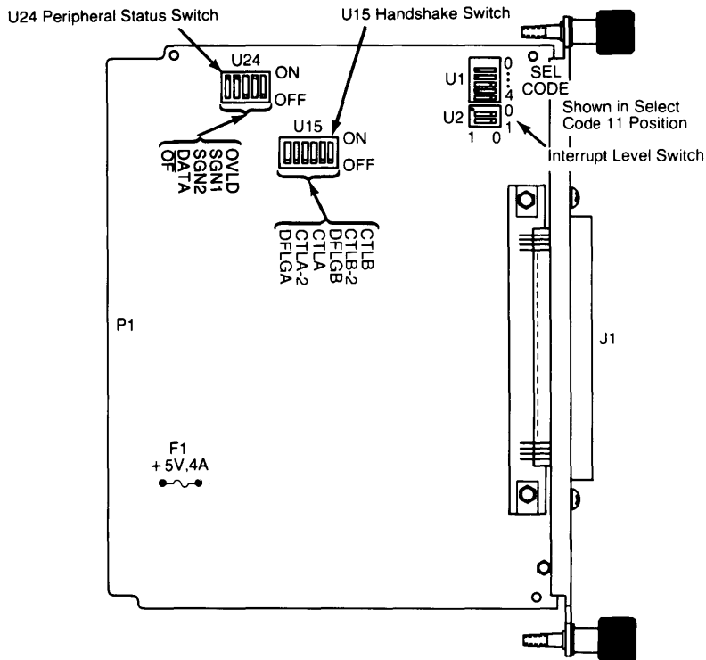
Figure 5-6. HP 98623A BCD Interface switches.
