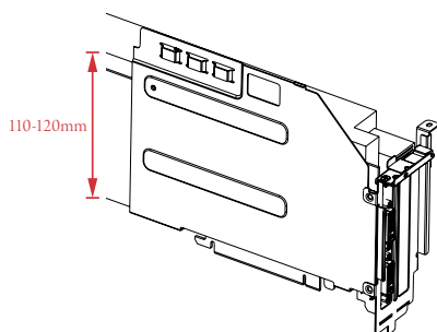
Standard-height card
