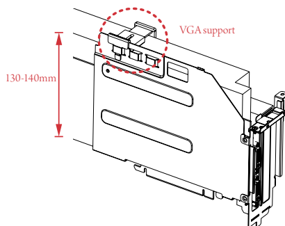
Over-height card
