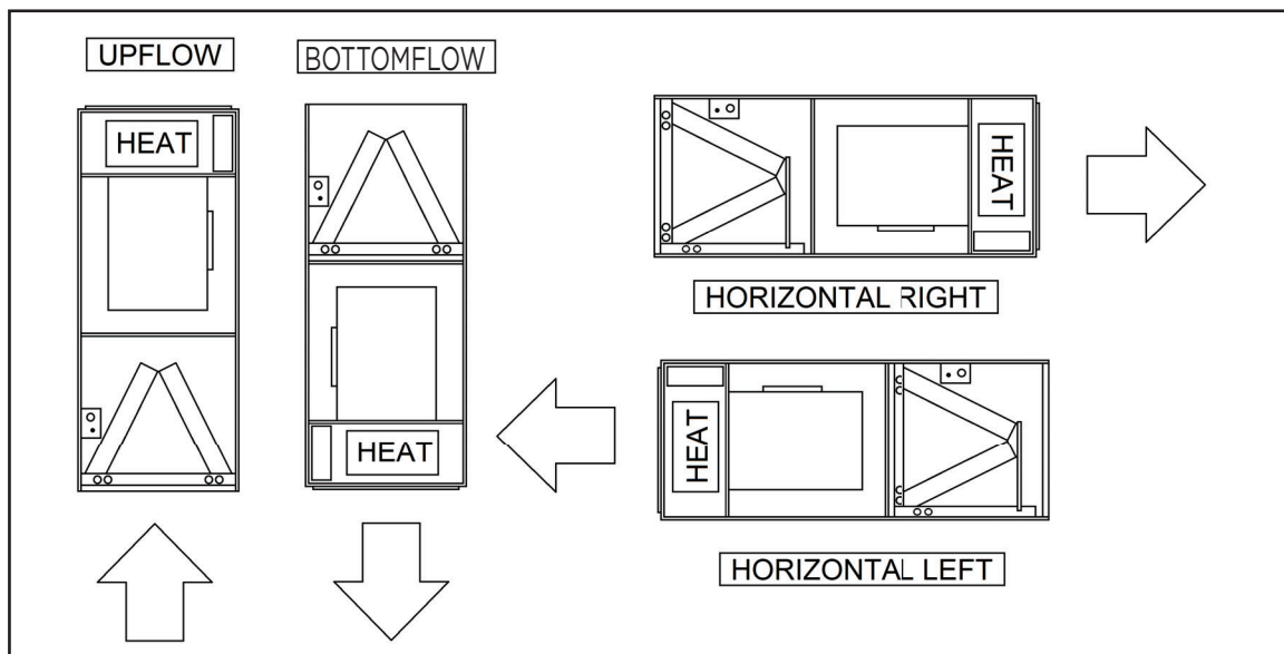
FIGURE 3: Typical Installation
