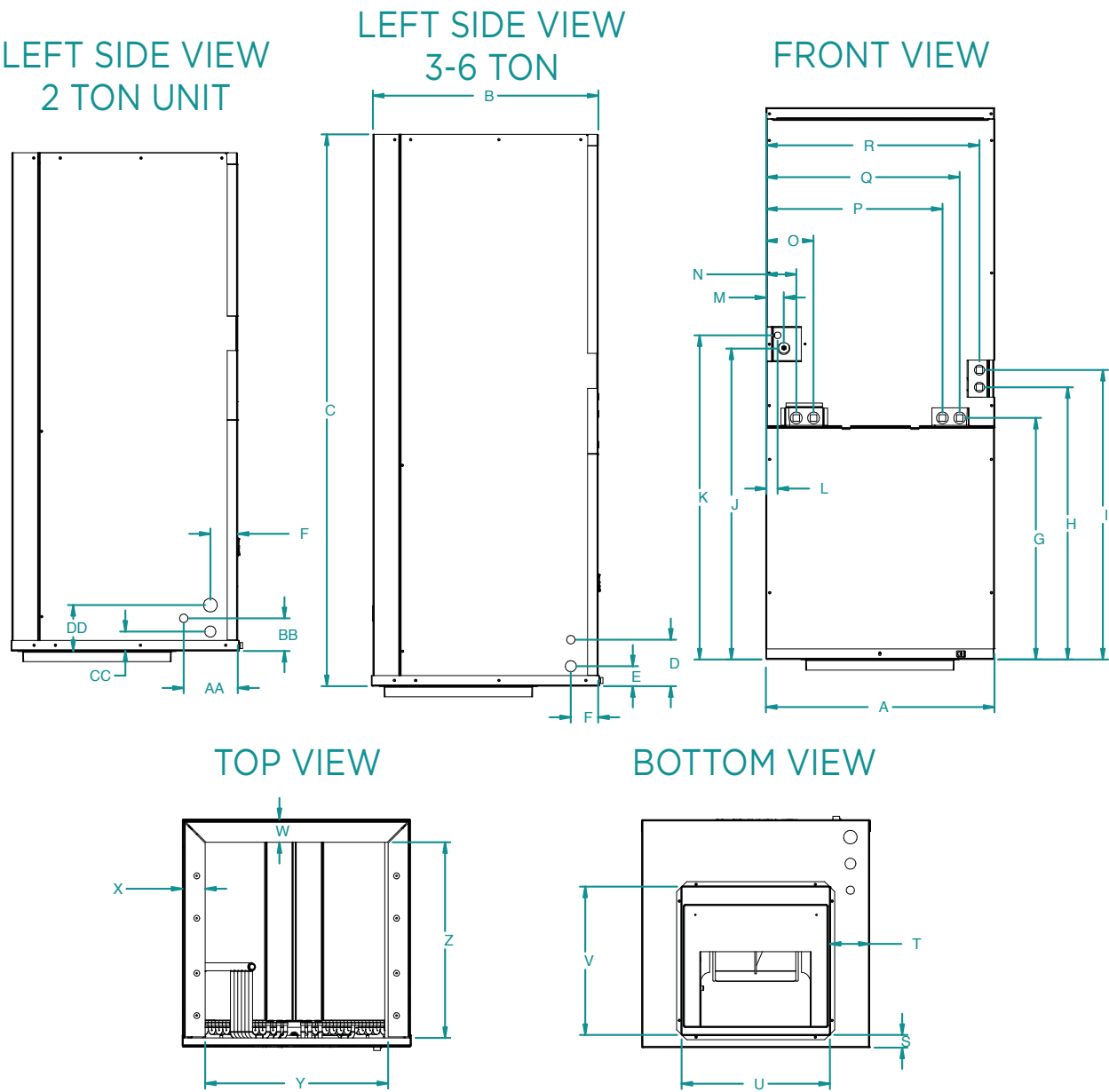
SAH Air Handler - Bottom flow
