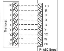
Non-Communicating Thermostat
