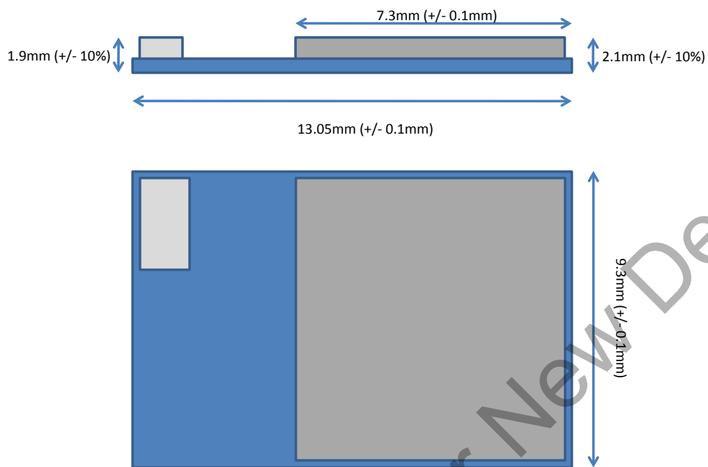
Figure 5: External dimensions
