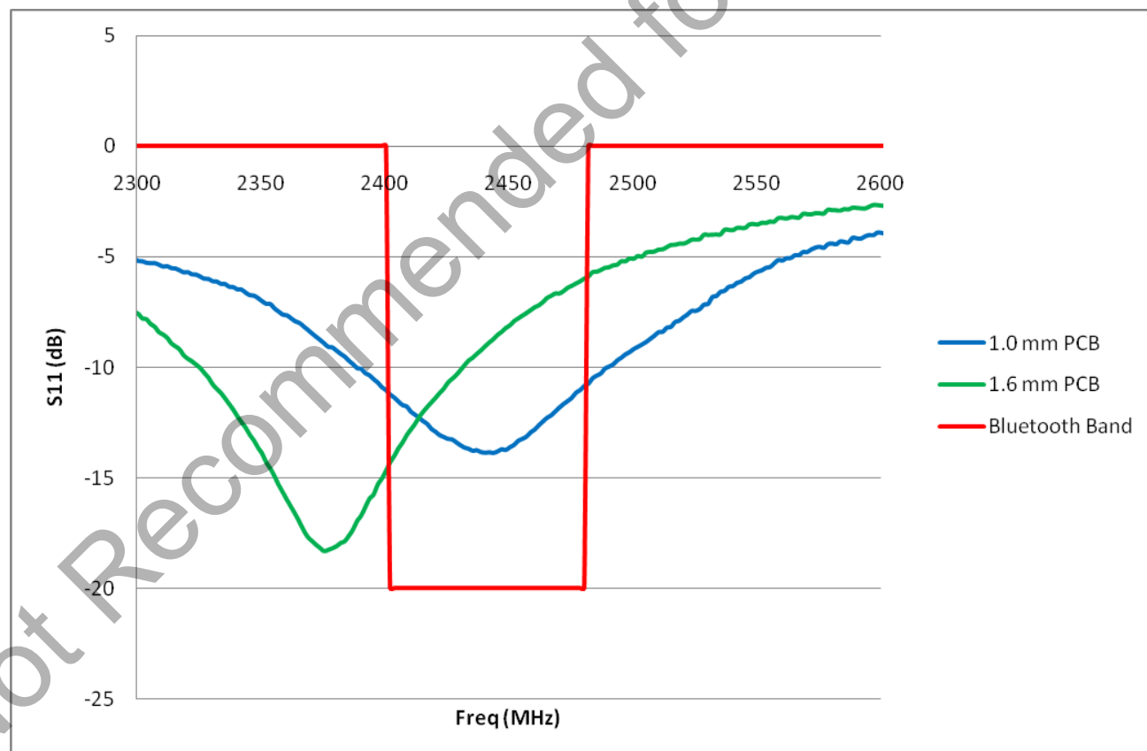
Figure 9: Impedance matching of the antenna of BT111 with two different mother board PCB thickness
