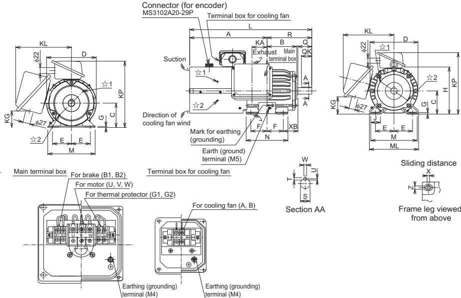
Frame Number 100L, 112M, 132S, 132M
