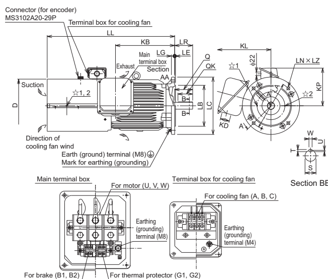
Frame Number 160M, 160L
