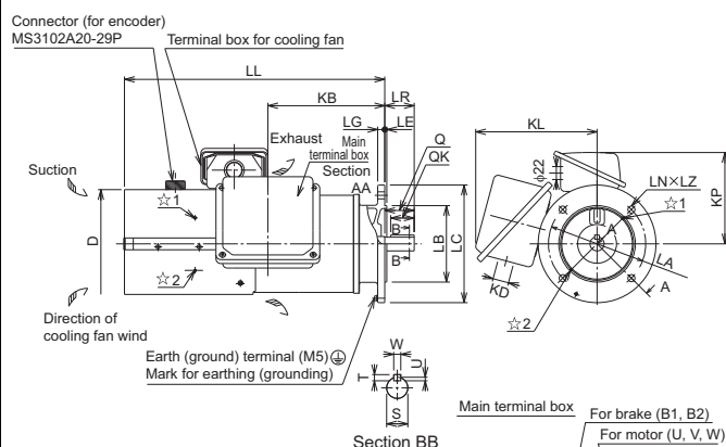
Frame Number 90L
