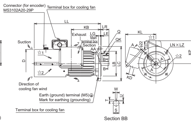
Frame Number 100L, 112M, 132S, 132M
