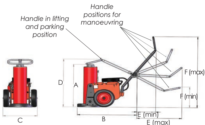
Dimensions for all other models:
