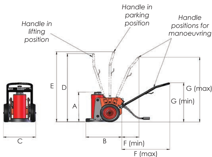
Dimensions for 50 tonne models:
