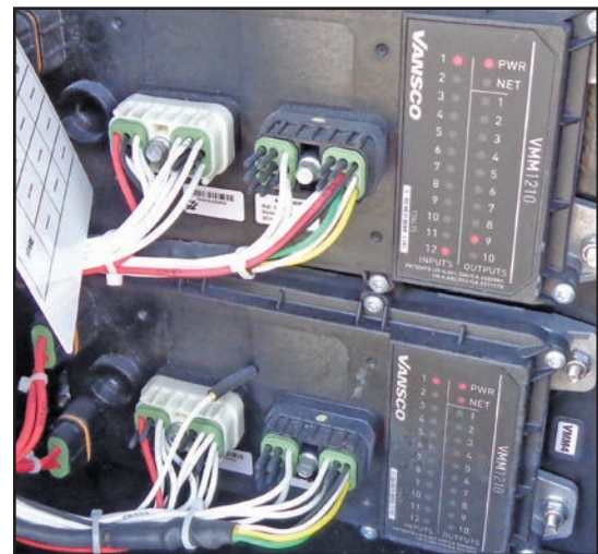
Figure 8-8: Multiplex system
