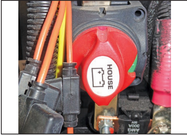
Figure 8-3: House batteries
