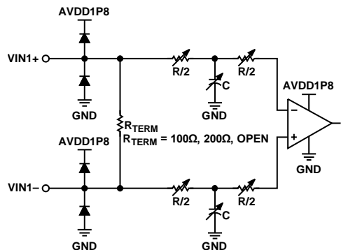
Figure 47. Analog Inputs
