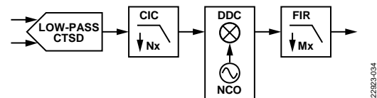
Figure 70. Simplified Diagram of the Digital Functional Block
