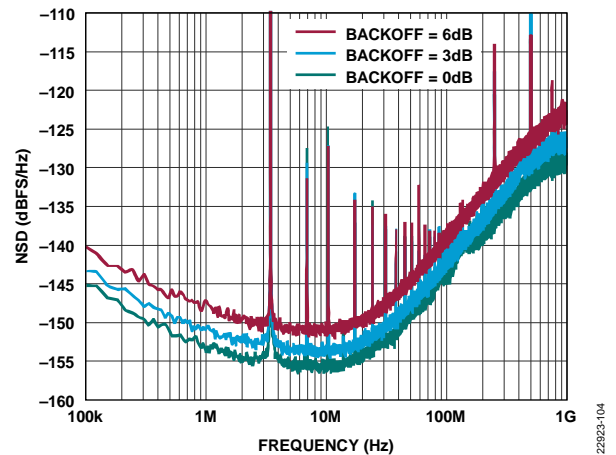
Figure 8. ADC NSD at Various Backoff Values, 2 GSPS
