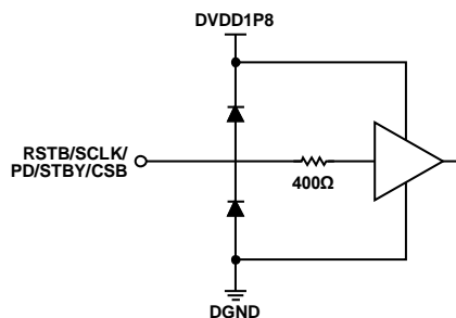
Figure 49. RSTB, SCLK, PD/STBY, and CSB Inputs
