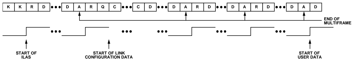
Figure 87. Initial Lane Alignment Sequence
