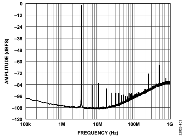
Figure 7. ADC Noise Floor at Backoff = 3 dB, 2 GSPS
