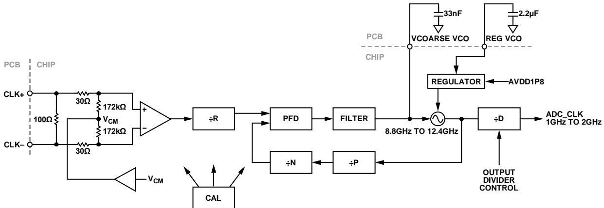
Figure 68. AD9083 Clock Path Block Diagram
