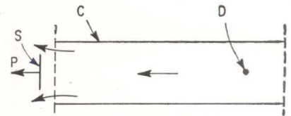
PRINCIPLE of new microwave power meter—Fig. 1
