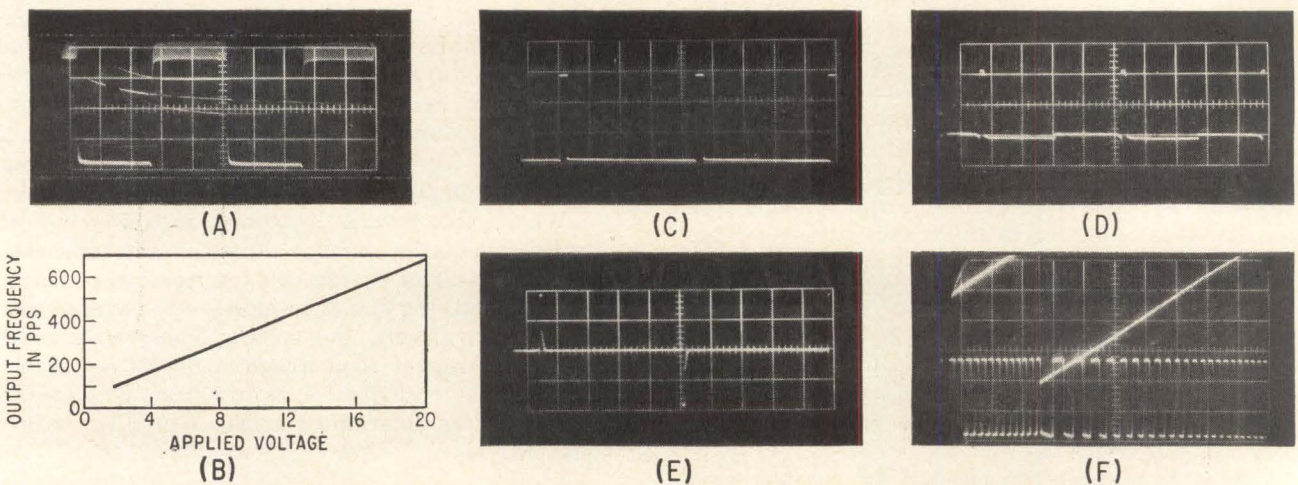
MULTIVIBRATOR running at 100-pps is locked to 100-kc input (A); converter linearity is better than 0.1 percent over 10:1 range (B); highly asymmetrical oscillator runs at 1-pps (C); one-shot is triggered at 1,160 pps (D); bistable circuit is driven at 1,090-pps (E); and five-to-one frequency sweep is produced by sawtooth input to converter (F)—Fig. 2
