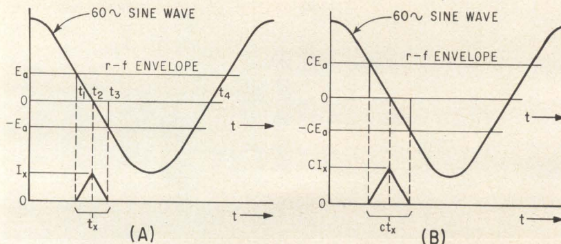
DIODE curve shows cutoff portion between 0 and t_1 (A) and current triangle (B)—Fig. 2
