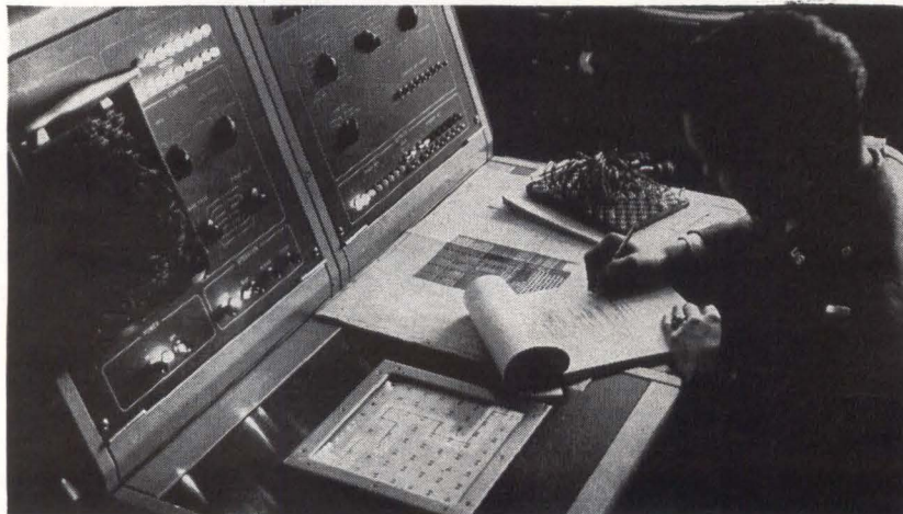
MAZE PROBLEM is run on Lannet (Large Artificial Nerve Network) developed by Melpar for Air Force and shown last week at the bionics symposium in Dayton, Ohio (p 8, March 22)
