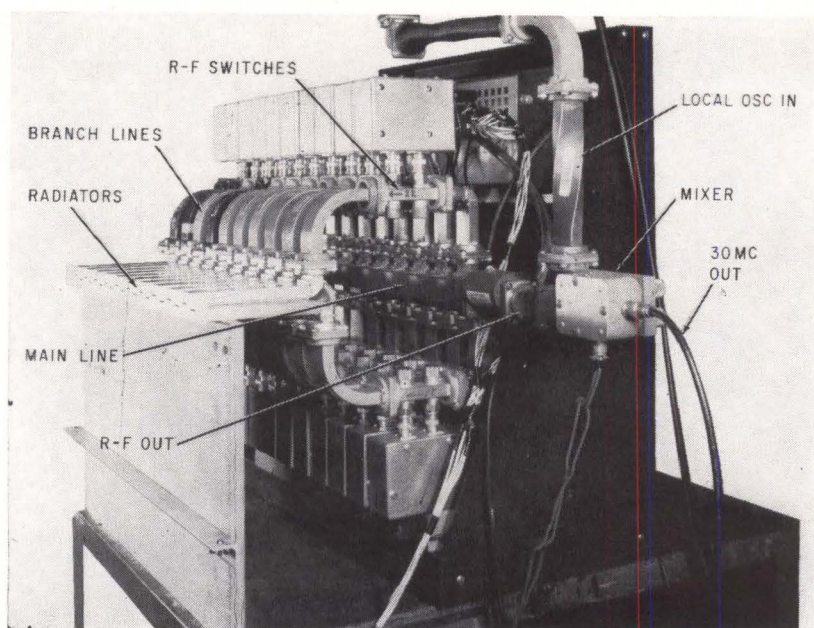
TWENTY-ELEMENT array
