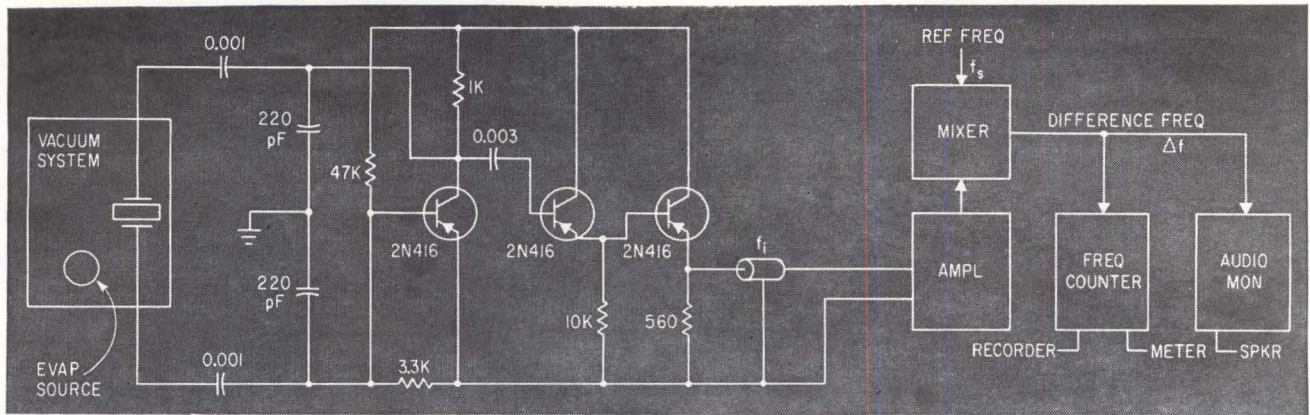
MONITOR crystal, mounted in same vacuum system as components being made, changes frequency with deposition thickness. Difference frequency output of mixer changes as crystal thickness increases—Fig. 1
