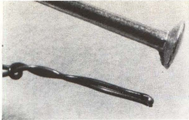
LASER WELD of 0.004-in.-diameter copper-constantan thermocouple. Hughes says wires need not be stripped
