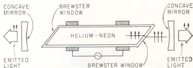
BASIC POSITION of mirrors in Hitachi laser
