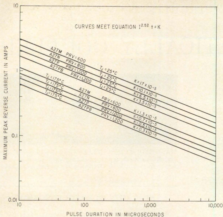
NONRECURRENT reverse current surge curve indicates capabilities of 12-ampere rectifier at different pulse durations—Fig. 2
