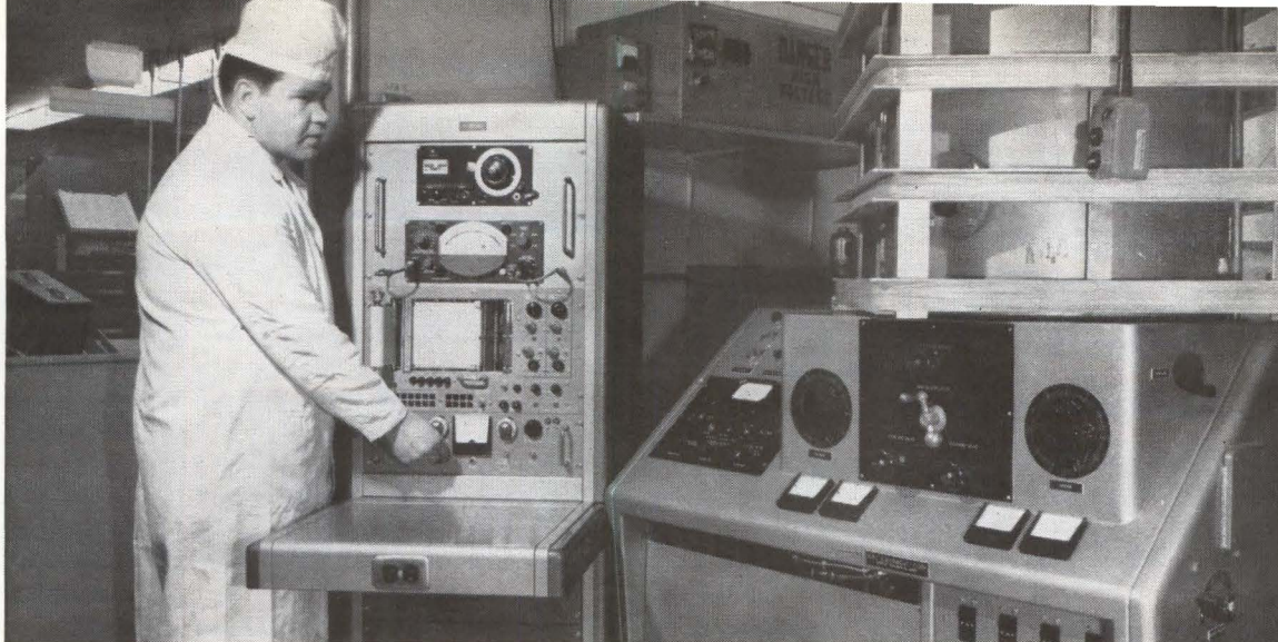
THIN-FILM thickness monitor deposition control equipment. Monitor oscillator is mounted below the vacuum-coater unit and thickness crystal is mounted within the vacuum system near the substrate
