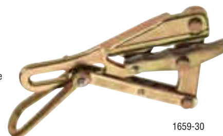
Serpentine Jaw
