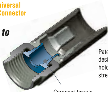
Compact ferrule
