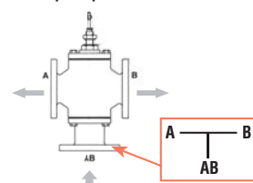
G7...D 3-way Diverting Valve Stem Up = Open AB to B
