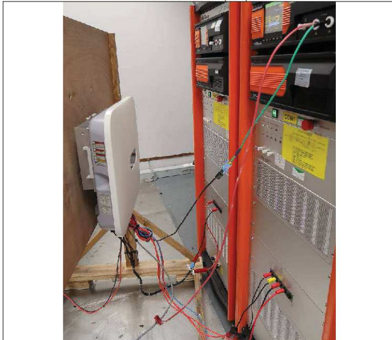
SURGE TEST (485)
