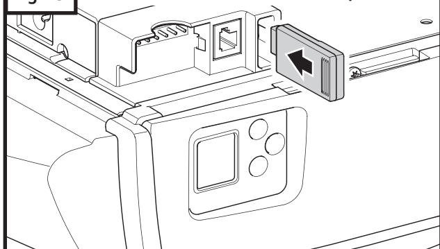
Fig. 43 Modular Antenna Installation or Replacement
