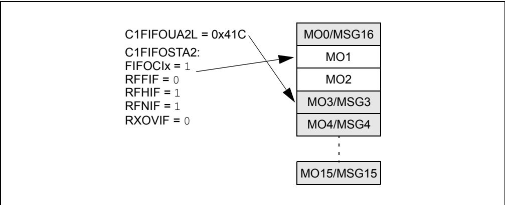
Figure 10-14: FIFO 2 – Two More Messages Read
