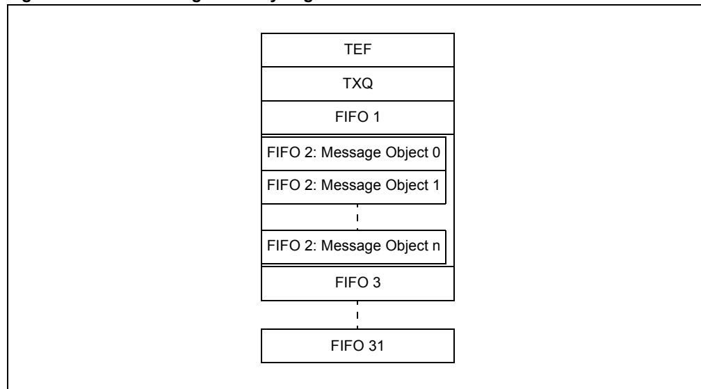
Figure 5-4: Message Memory Organization
