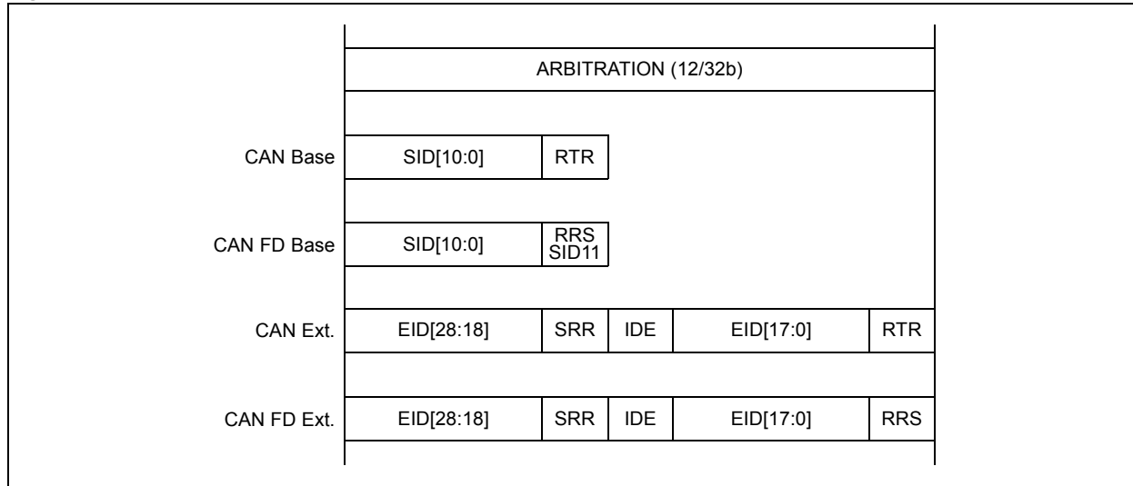
Figure 2-2: Arbitration Field
