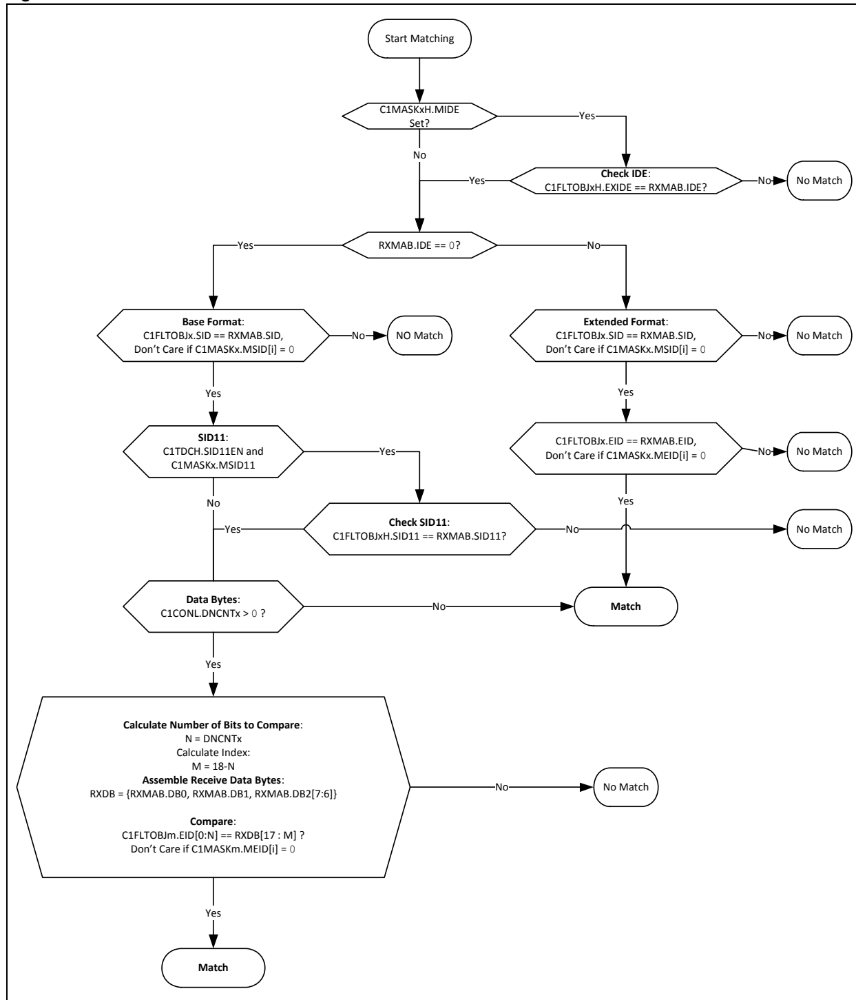
Figure 8-2: Filter Match
