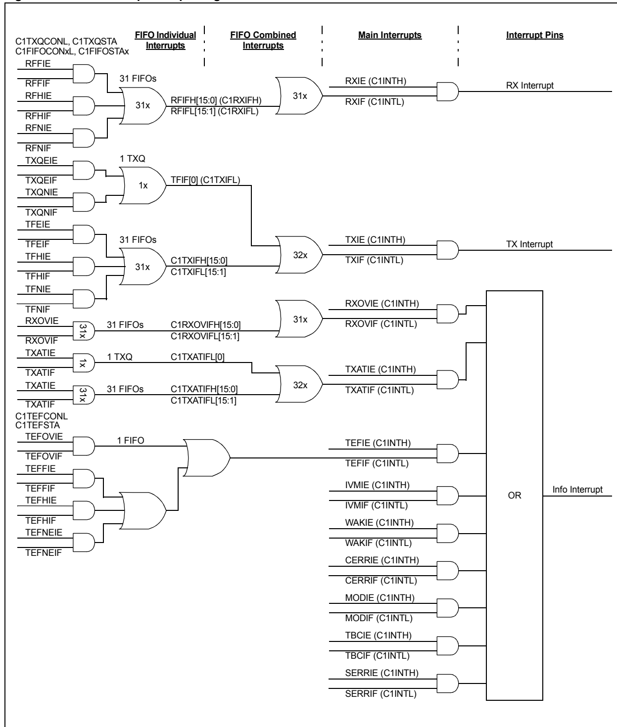
Figure 12-1: Interrupt Multiplexing
