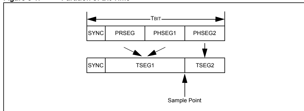
Figure 5-1: Partition of Bit Time
