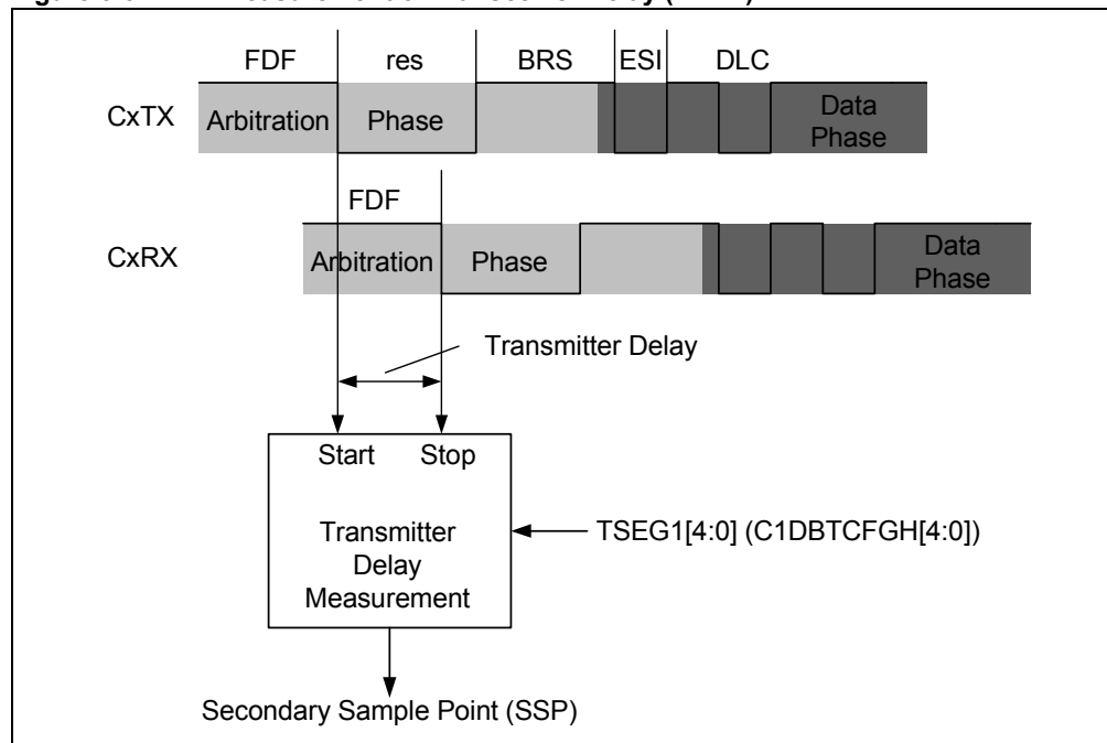
Figure 5-3: Measurement of Transceiver Delay (TDCV)
