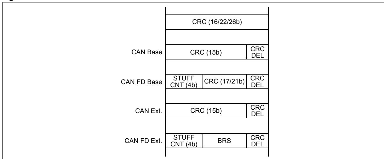
Figure 2-4: ISO CRC Field
