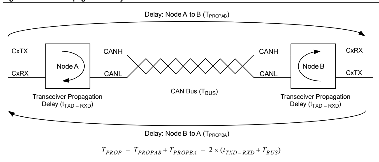
Figure 5-2: Propagation Delay
