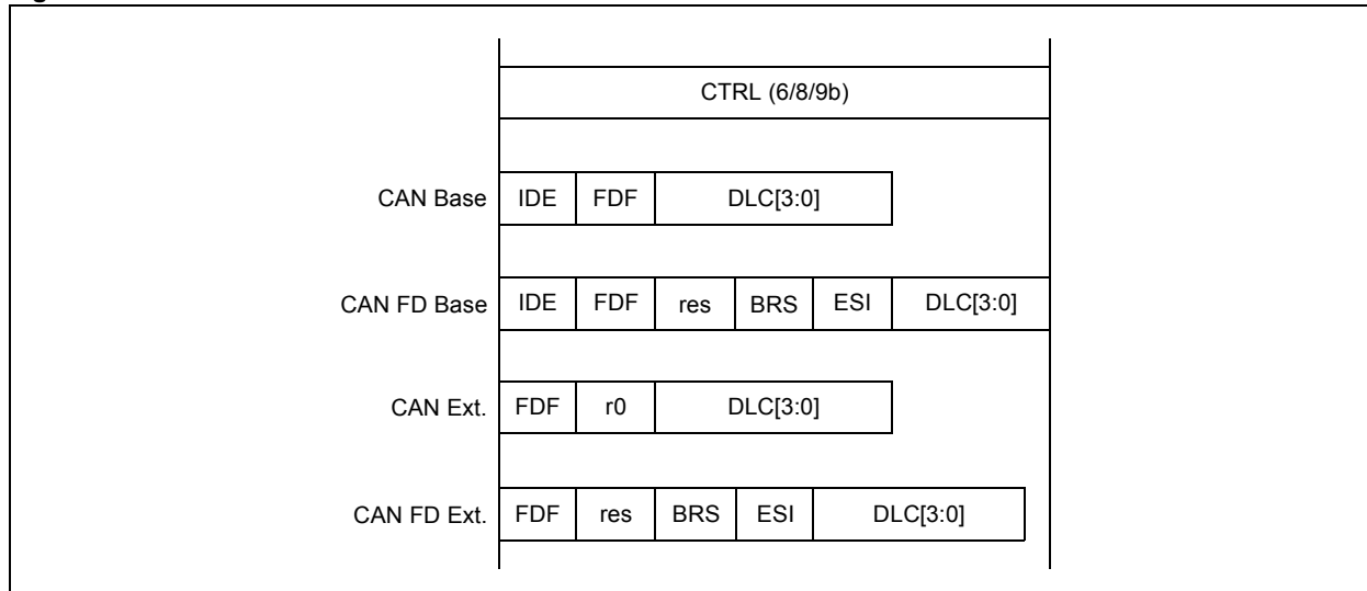
Figure 2-3: Control Field
