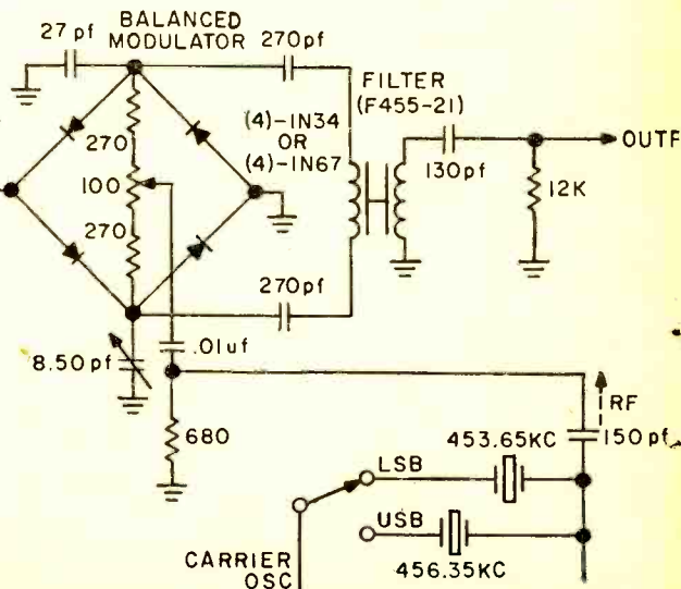
Fig. 8. Filtering circuit uses a 4-diode balanced modulator. The RF signal is generated by one of the two crystals, one for each sideband. The RF is fed up to the center of the modulator, and phasing of the signal cancels the RF. But when audio is applied to the modulator, the resulting imbalance allows RF to appear in the output. This RF is a double-sideband signal, minus the steady carrier. To get rid of one sideband, the composite signal passes through the filter. The resulting single-sideband signal is heterodyned in the transmitter's later stages, up to the final operating frequency of 27 MHz.
