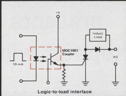
Logic-to-load interface Type: MOC1001 Coupler Price: $1.95 Features: 2,500 V Isolation 60% Transfer Ratio
