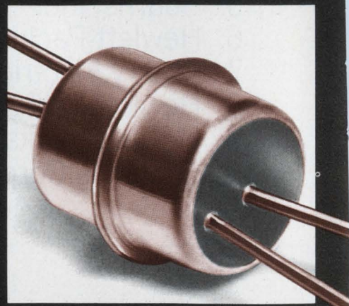
Type: MOC1002 Coupler Price: $1.50 Features: 1,500 V Isolation 30% Transfer Ratio
