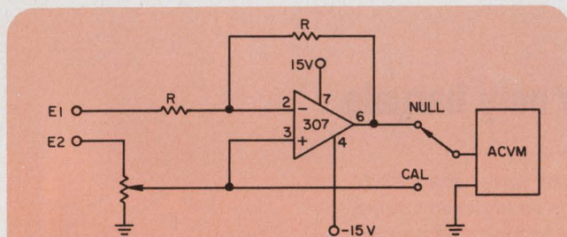
The phase angle between E_1 and E_2 may be determined by measuring signal magnitudes in the null and "cal" positions. Before measurements are taken, the potentiometer is adjusted for a minimum signal at the op-amp output.
