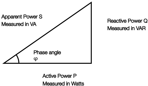
Figure 3.2 – The power triangle diagram
