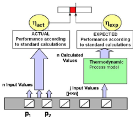
Figure 4.9 – Simulation and monitoring with PowerCycle software, (ABB Switzerland, Power Technology Systems, 2005, PowerCycle brochure)
