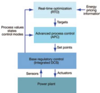
Figure 4.8 – Multi-level real-time optimization, (Immonen, Coordinated Control and Optimization of a Complex Industrial Power Plant, 2008)
