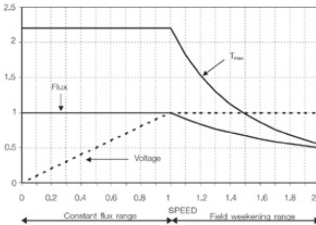
Figure 2.31 - Torque-speed curves for idealized VFD, (ABB Drives 2002)
