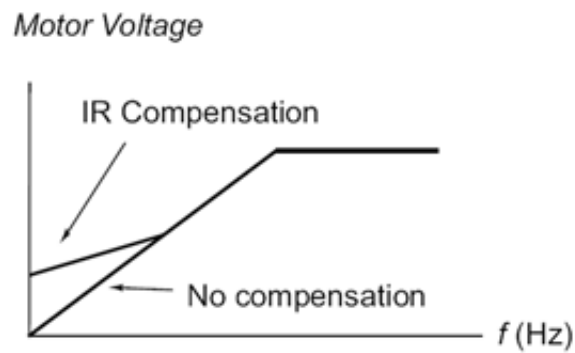
Figure 2.34 – Voltage boost at low speed, ABB VFD Programmable Features
