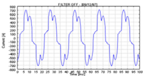
Figure 3.8 – Graph of high harmonic content 50 Hz waveform, (ABB Kurt Schipman)
