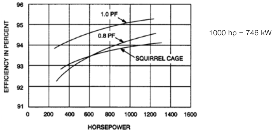
Figure 2.21 - Typical Full Load Efficiencies for synchronous vs. induction motors, (IEEE, 2007)
