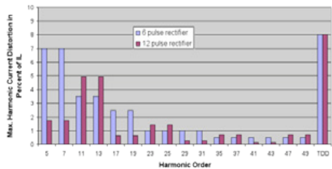
Figure 3.13 – Harmonic distortion for 6 and 12 pulse rectifiers, (ABB Industrie AG, 2006)
