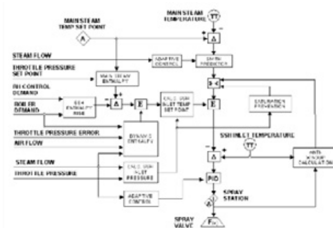
Figure 5.13 - Advanced Steam Temperature control system logic, (ABB Inc. Plant Automation, 2006)
