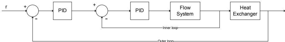
Figure 4.6 – Cascade feedback controller block diagram
