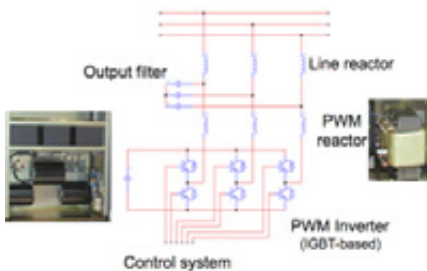
Figure 3.12 – Active filter schematic, (ABB, Schipman, 2008)
