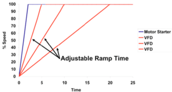
Figure 2.46 - VFD adjustable startup- speed vs. startup time, (ABB Oy. Drives, 2002)
