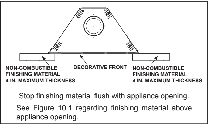
Figure 10.4 Non-Combustible Finishing Material
