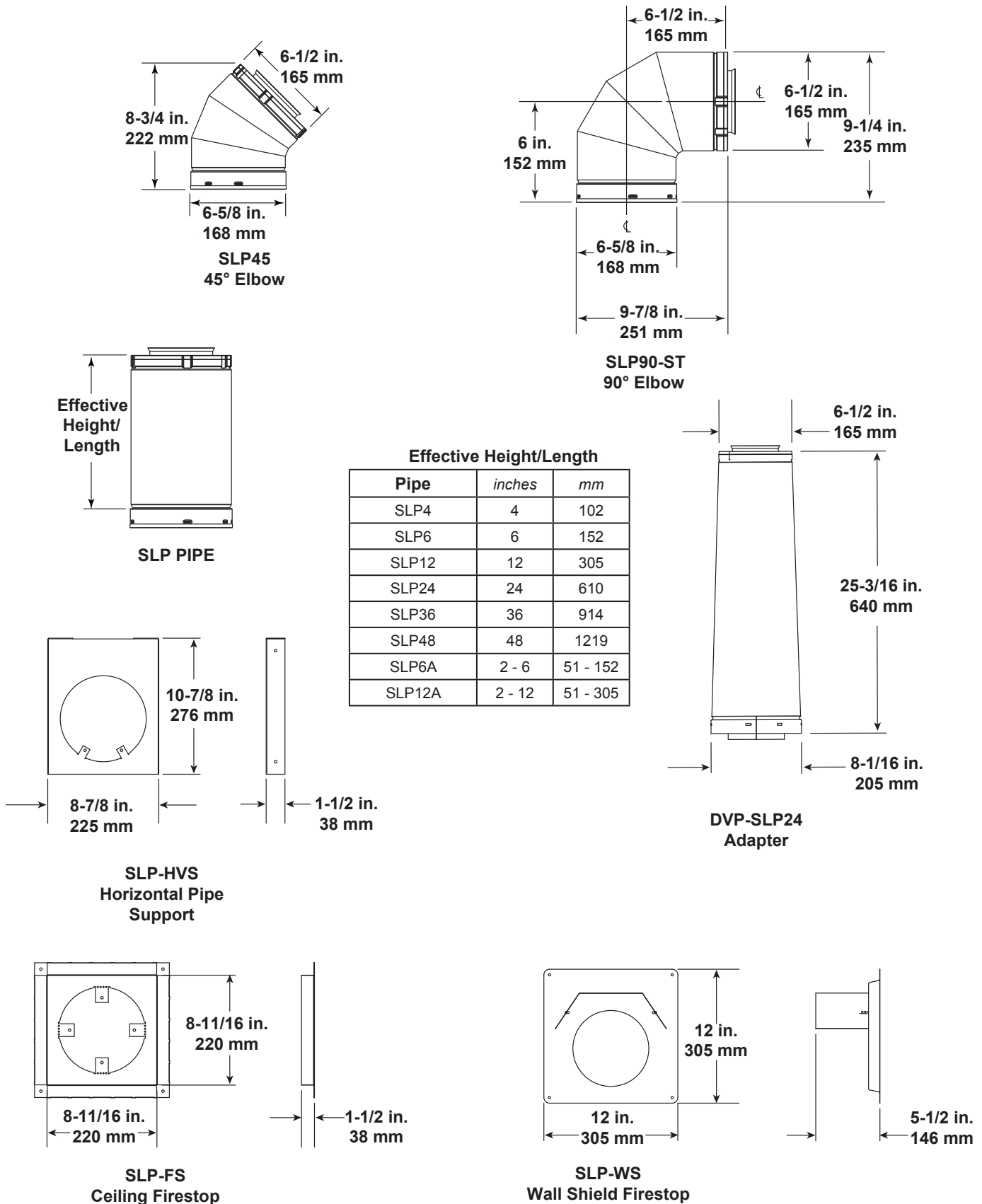
Figure 12.8 SLP Series Vent Components
