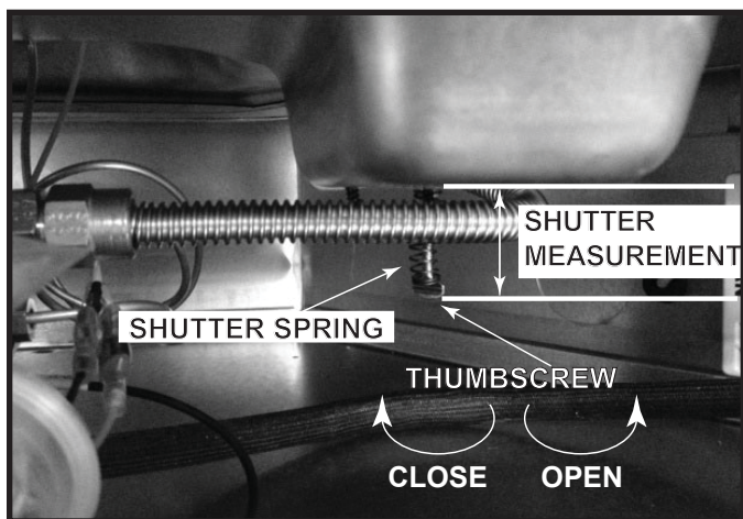
Figure 9.1 Air Shutter
