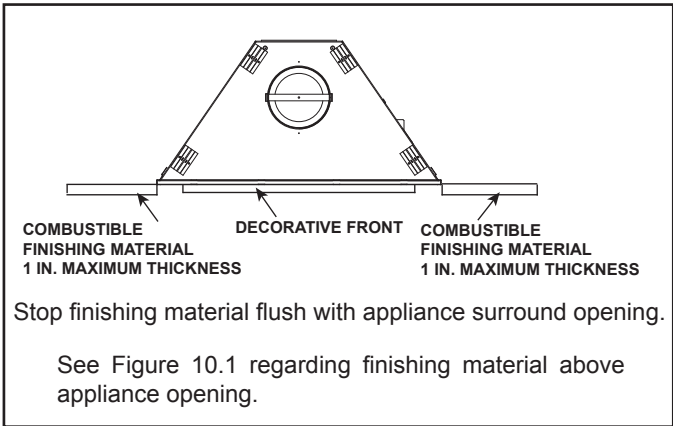
Figure 10.5 Combustible Finishing Material
