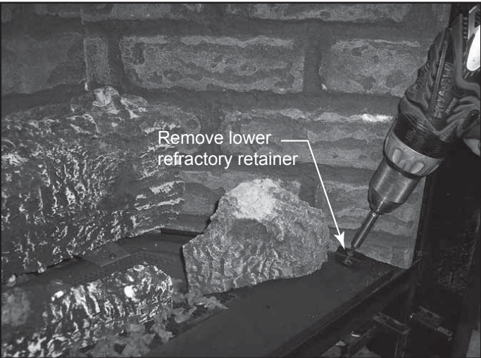
Figure 4.11a Remove Refractory Retainer
