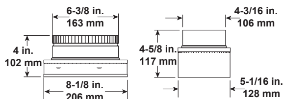
DVP-2SL Adapter
