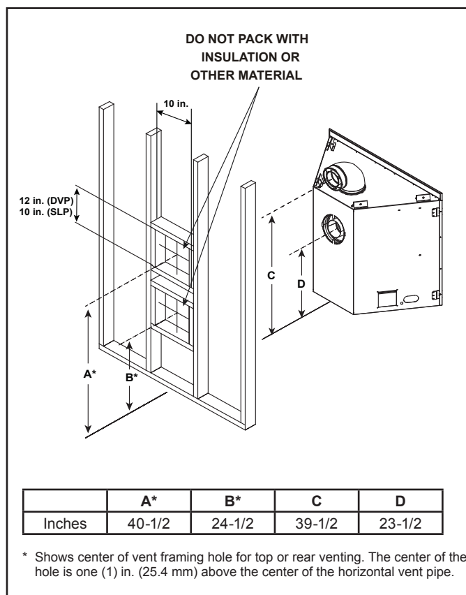
Figure 5.2 Wall Penetration
