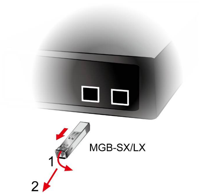
Figure 2-2-5: How to Pull Out the SFP/SFP+ Transceiver
