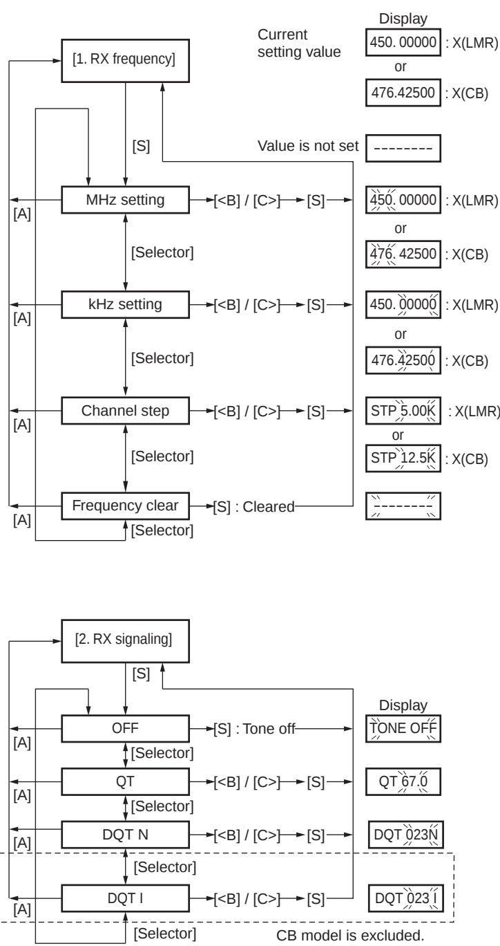
■ Item setting mode flow chart
