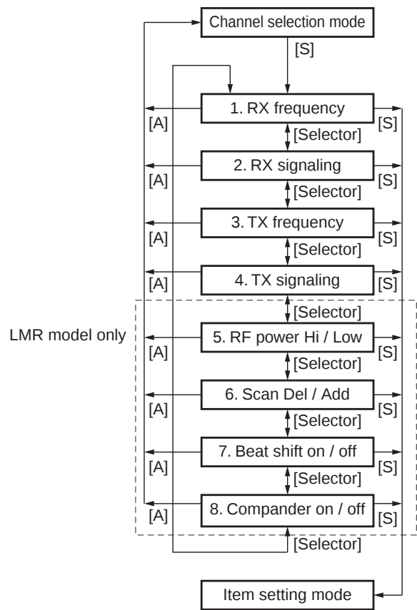
■ Item selection mode flow chart
