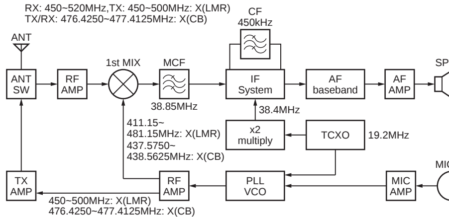
Fig. 1 Frequency configuration
