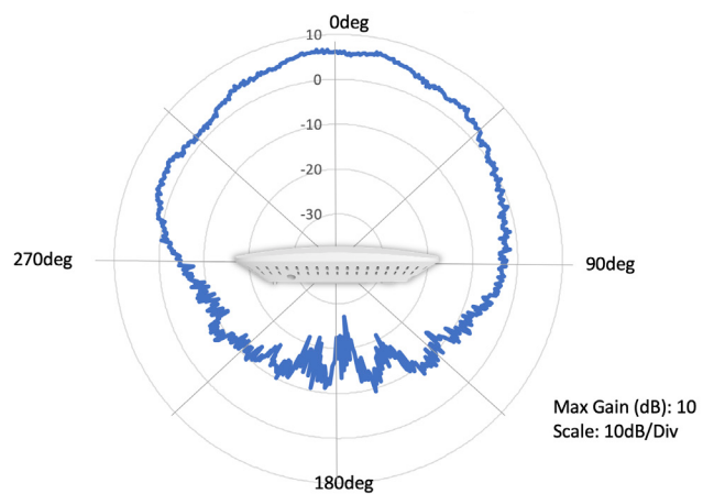
5 GHz Elevation
