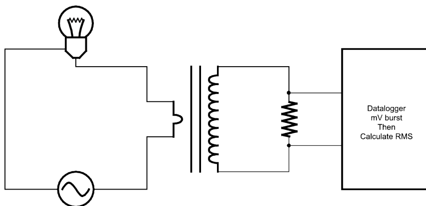
FIGURE C-2. Schematic of generator with current transformer
