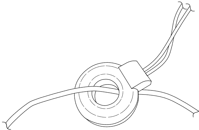
FIGURE C-4. CS11 with the AC wire
