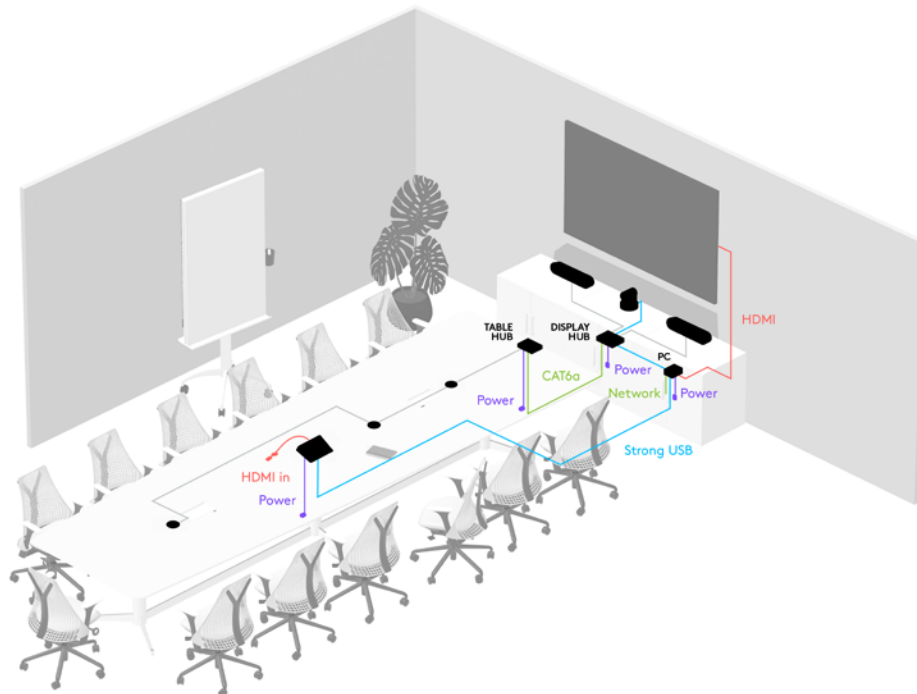
Large conference room cabling example with Logitech Rally ConferenceCam, Logitech Tap meeting room controller and dedicated room compute.
