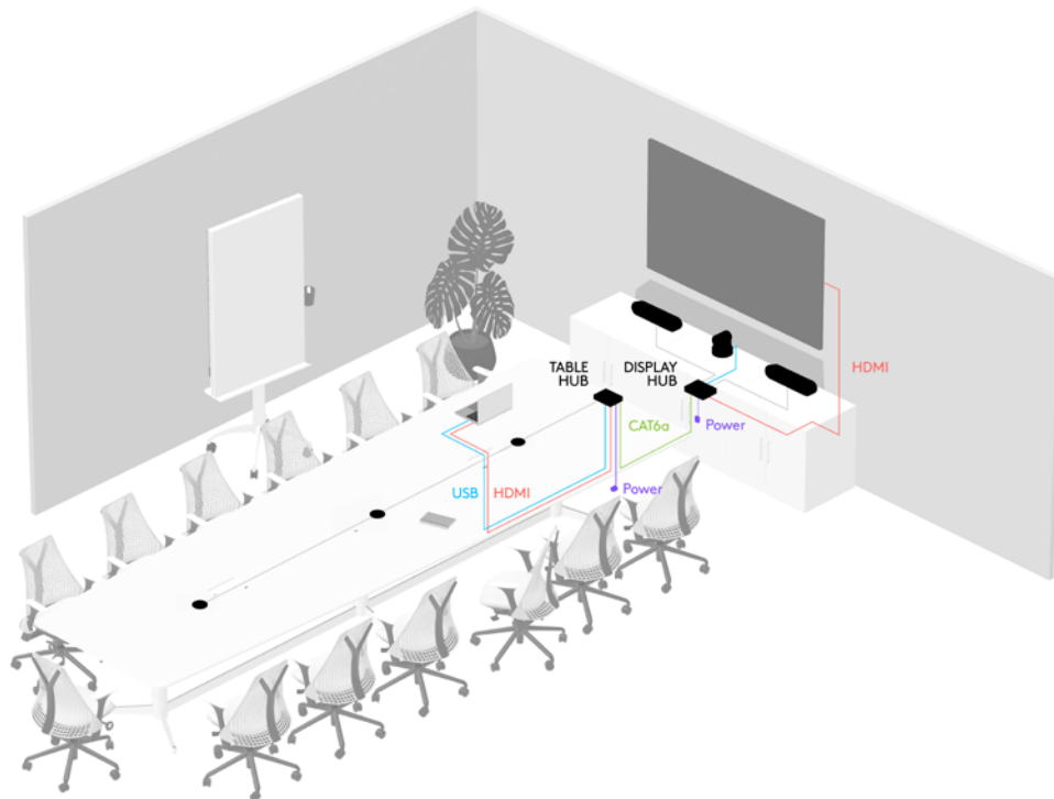
Large meeting room/boardroom cabling example with Rally and BYOD setup.
