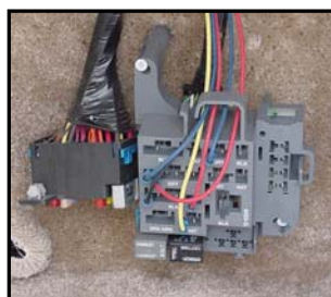
Figure 7-12. Fuse Blocks
