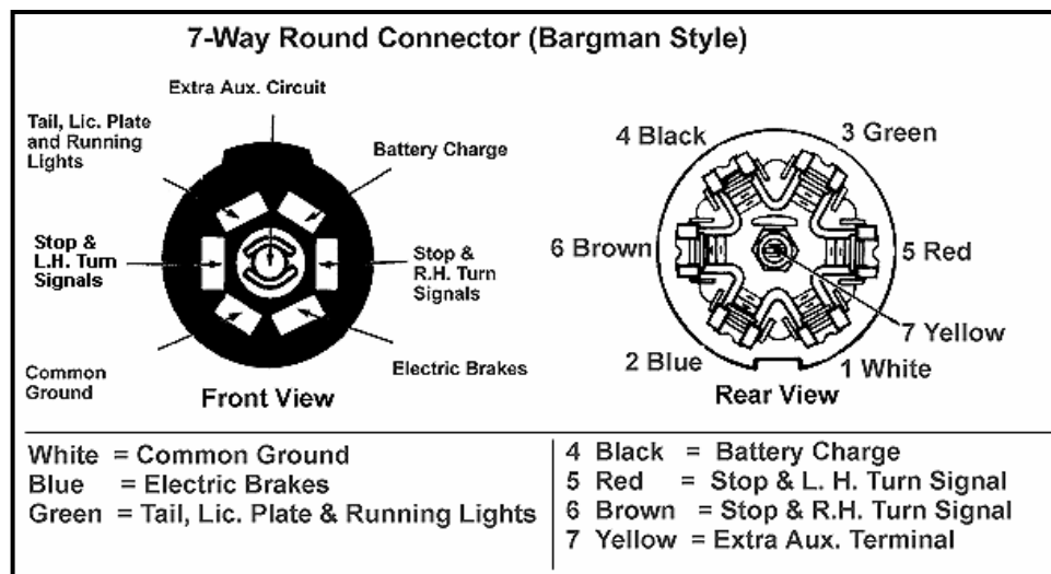
Figure 7-14. Seven-Pin Towing Connector
