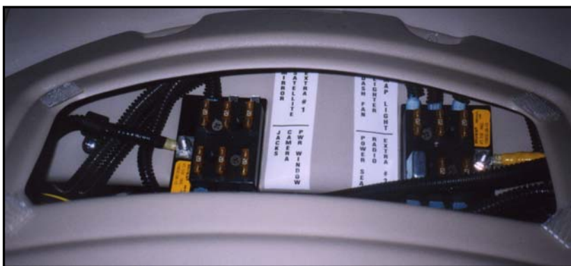
Figure 7-13. In-Dashboard Fuse Blocks
