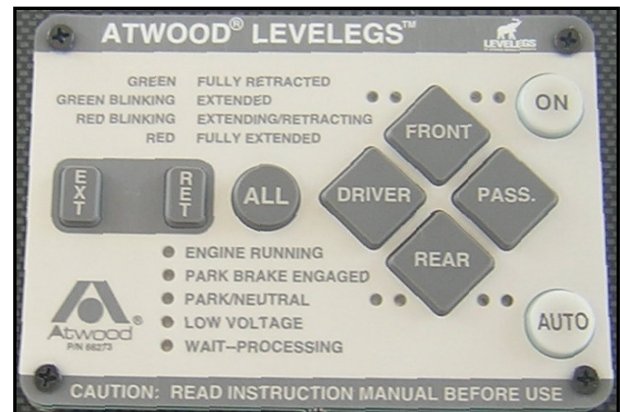
Figure 9-5. Leveling Control Panel on Dashboard
